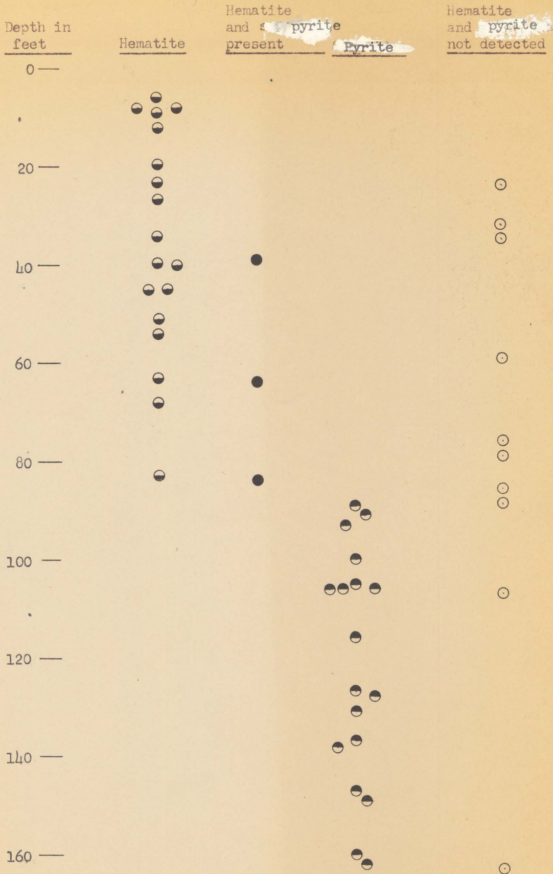
Figure 2. The subsurface occurrence of hematite and pyrite noted in the study of 49 thin sections from core taken from the Clarabelle area, Fall River County, South Dakota.
