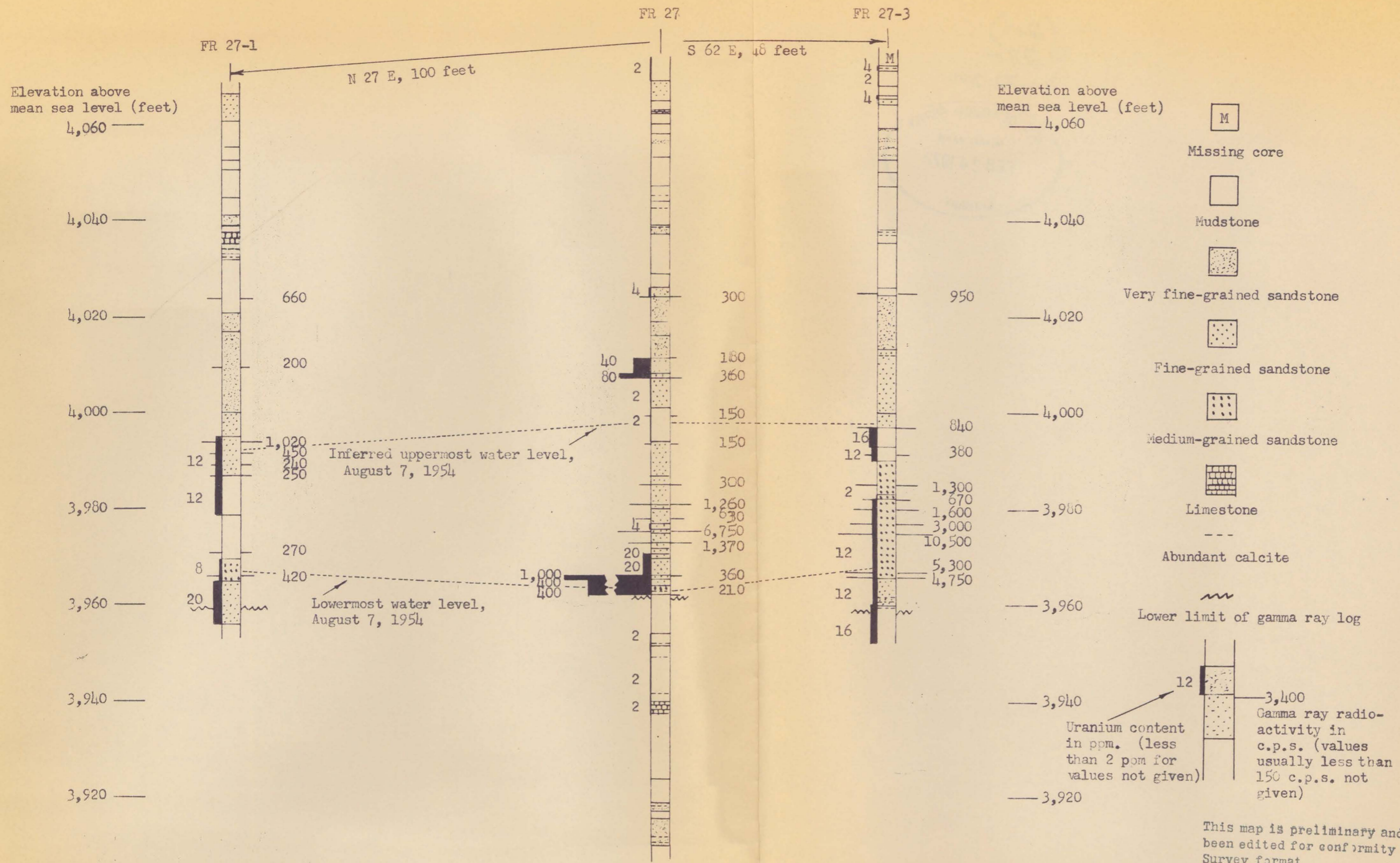
PLATE 9. CROSS SECTION SHOWING THE LITHOLOGY, GAMMA RAY RADIOACTIVITIES, URANIUM ANALYSES, AND WATER LEVEL BETWEEN A. E. C. DRILL HOLES FR 27-1, FR 27, AND FR 27-3 IN THE CLARABELLE AREA, FALL RIVER COUNTY, SOUTH DAKOTA
