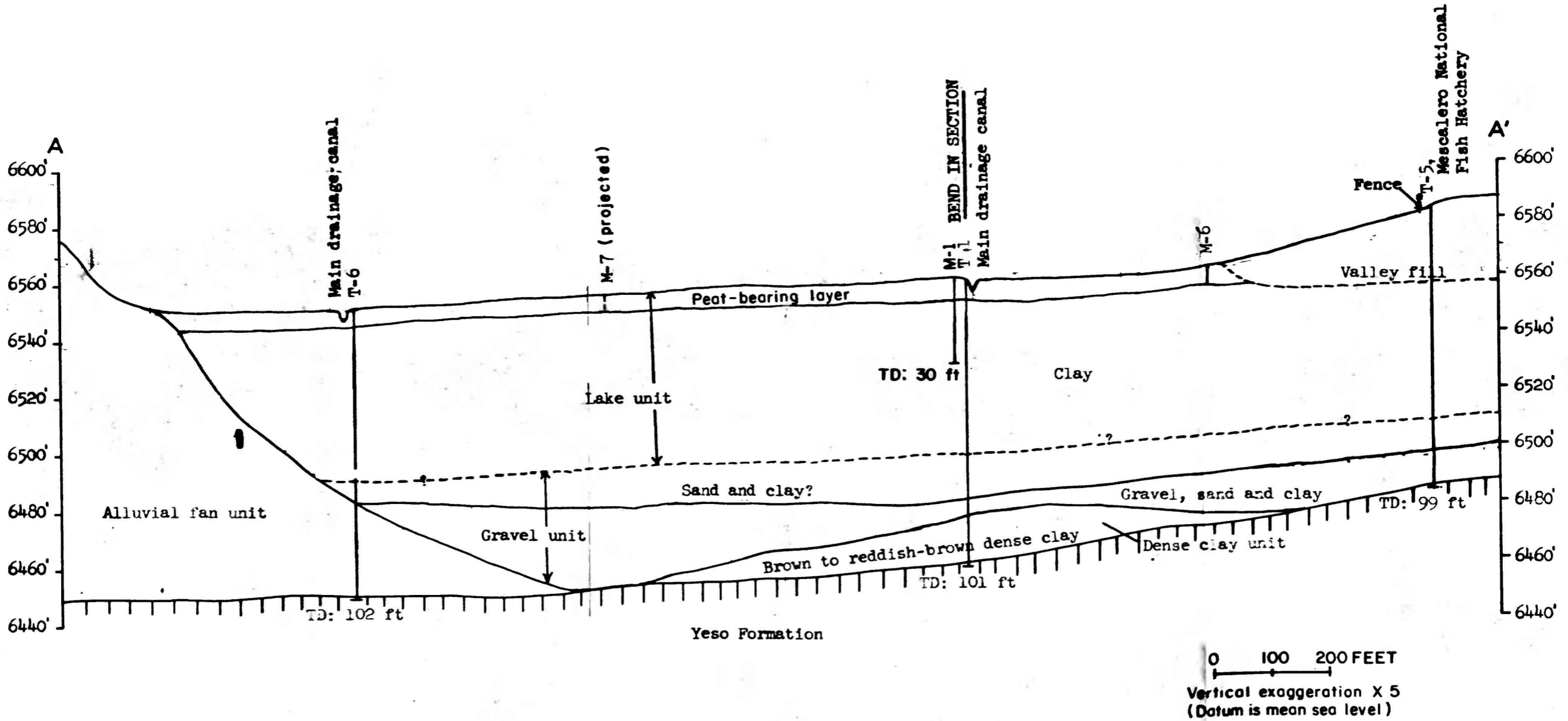
Figure 4. Section A-A' showing stratigraphic relations of unconsolidated deposits near Mescalero, Otero County, New Mexico.
