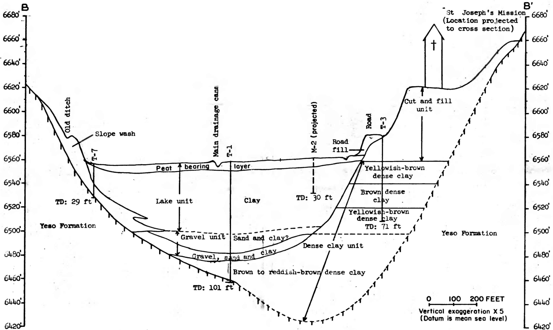
Figure 5. Section B-B' showing stratigraphic relations of unconsolidated deposits near Mescalero, Otero County, New Mexico.
