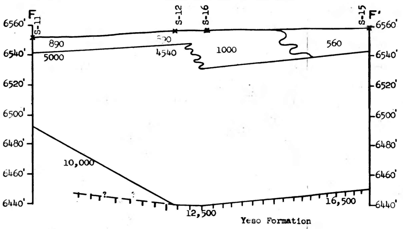
Figure 6.--Seismic sections C-C', D-D', E-E', and F-F' showing velocity interfaces in valley fill and depth to bedrock near Mescolero, Otero County, New Mexico.
