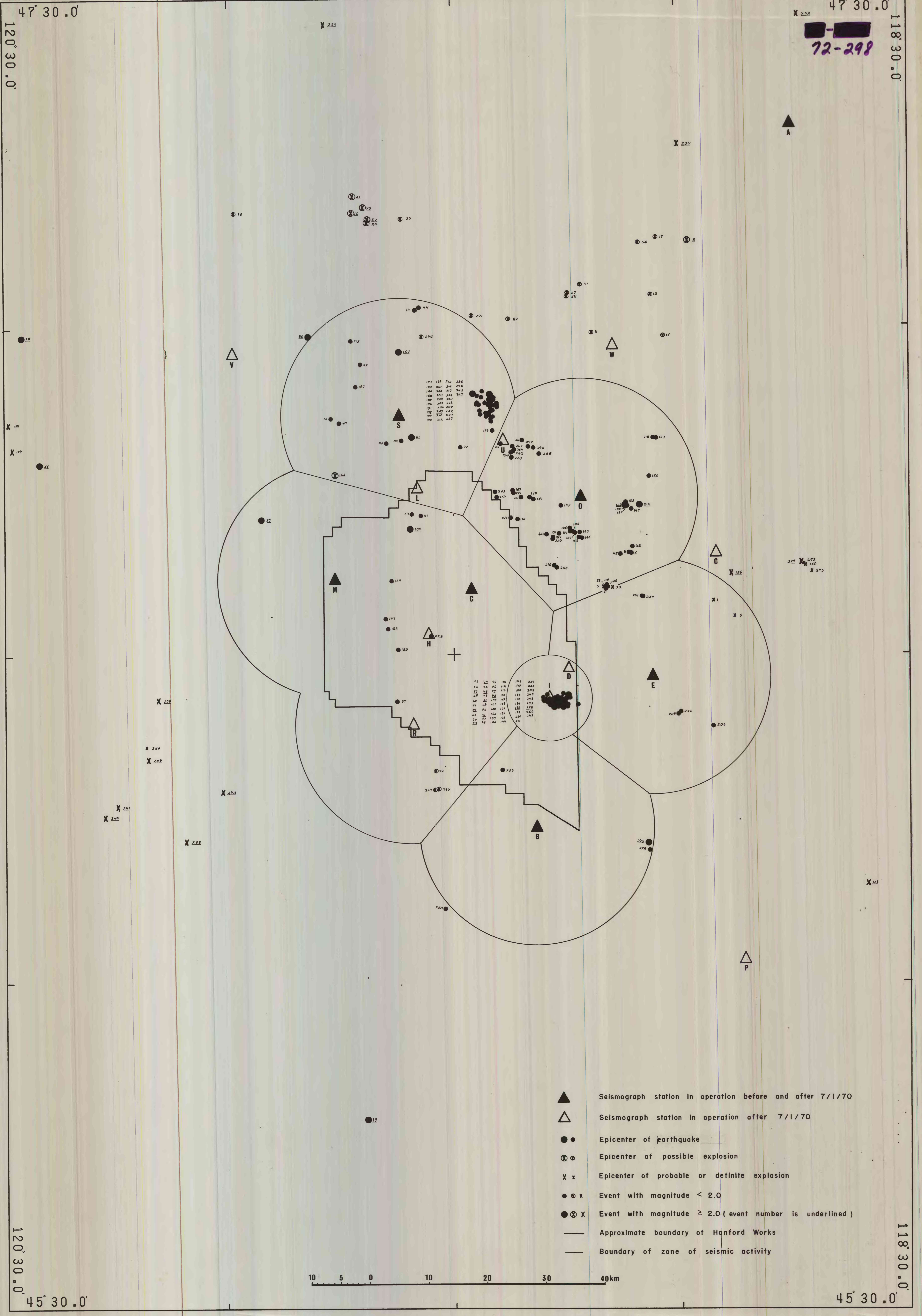
Figure 2. — Hanford region seismic events from March 23, 1969 to June 30, 1970
