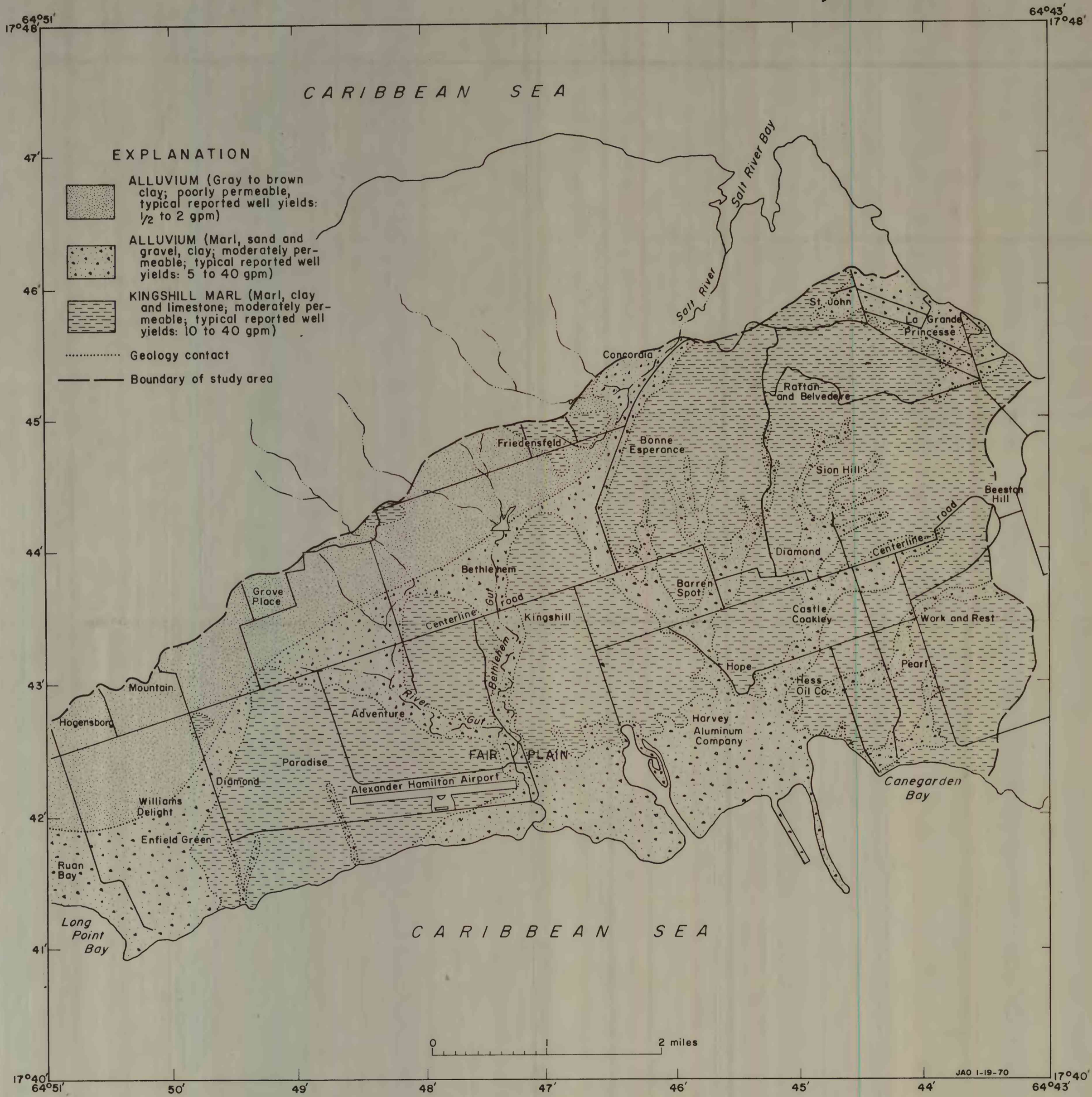
Figure 2.--Hydrogeology of central St. Croix, V.I. Modified from Cederstrom (1950) and Whetten (1966).
