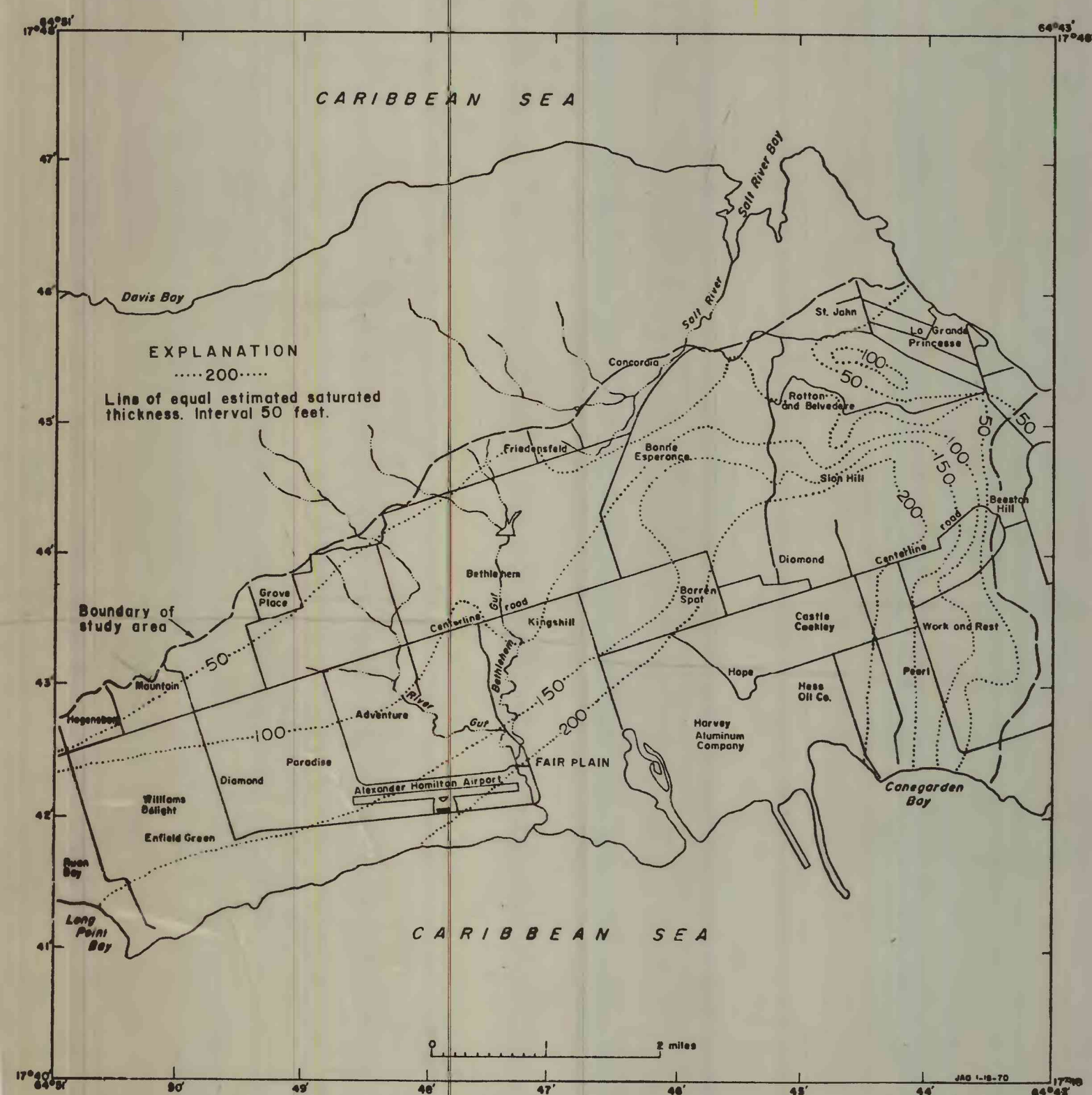
Figure 4.--Estimated saturated thickness of the Kingshill Marl and the associated alluvium in central St. Croix, V.I. (Spring 1968).
