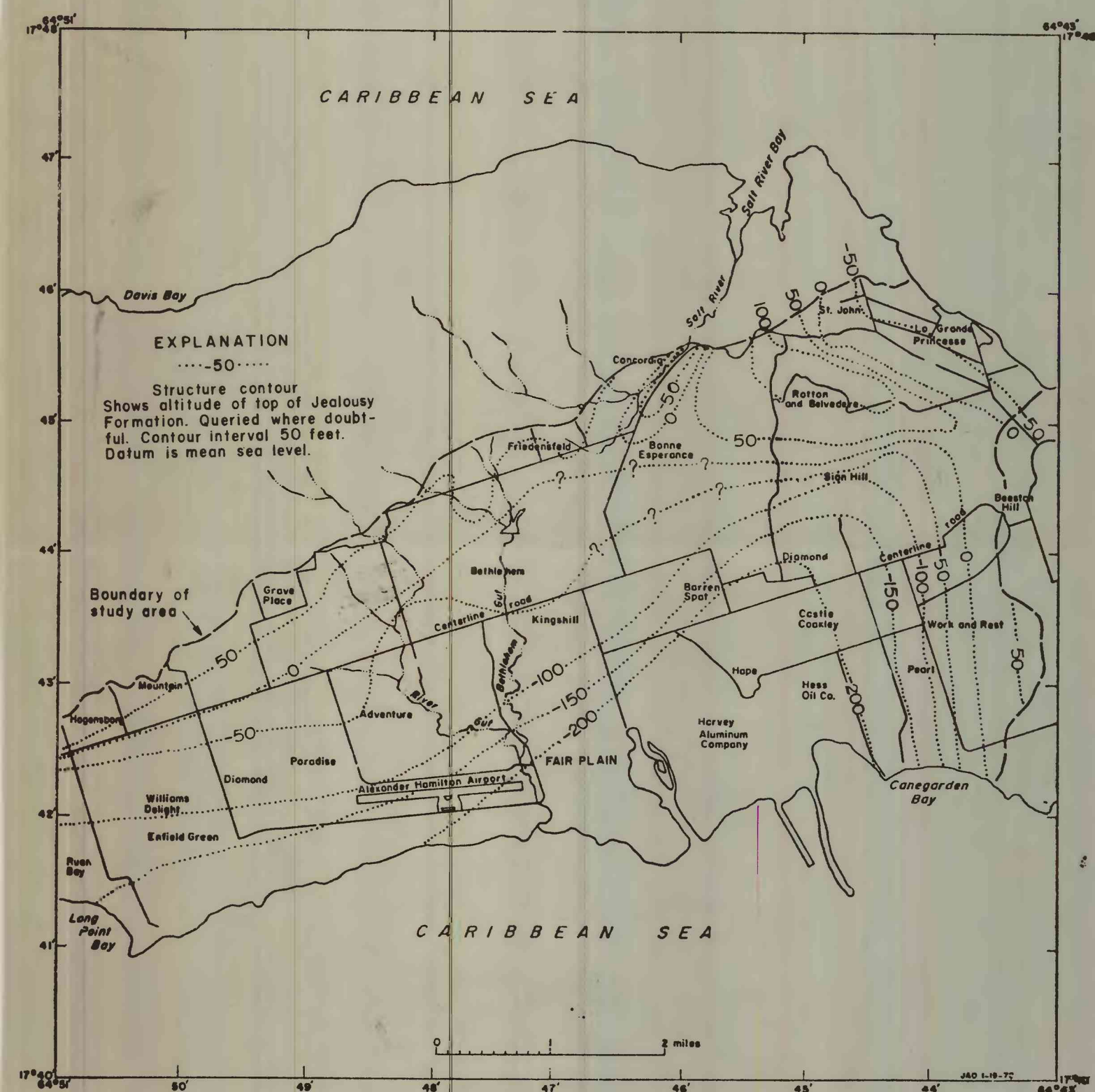
Figure 3.--Estimated altitude of the top of the Jealousy Formation ("blue clay") in central St. Croix, V.I.
