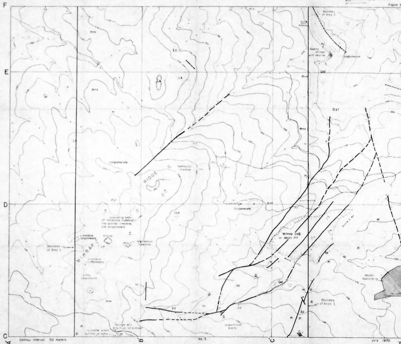
GEOLOGIC MAP OF AREA 1
