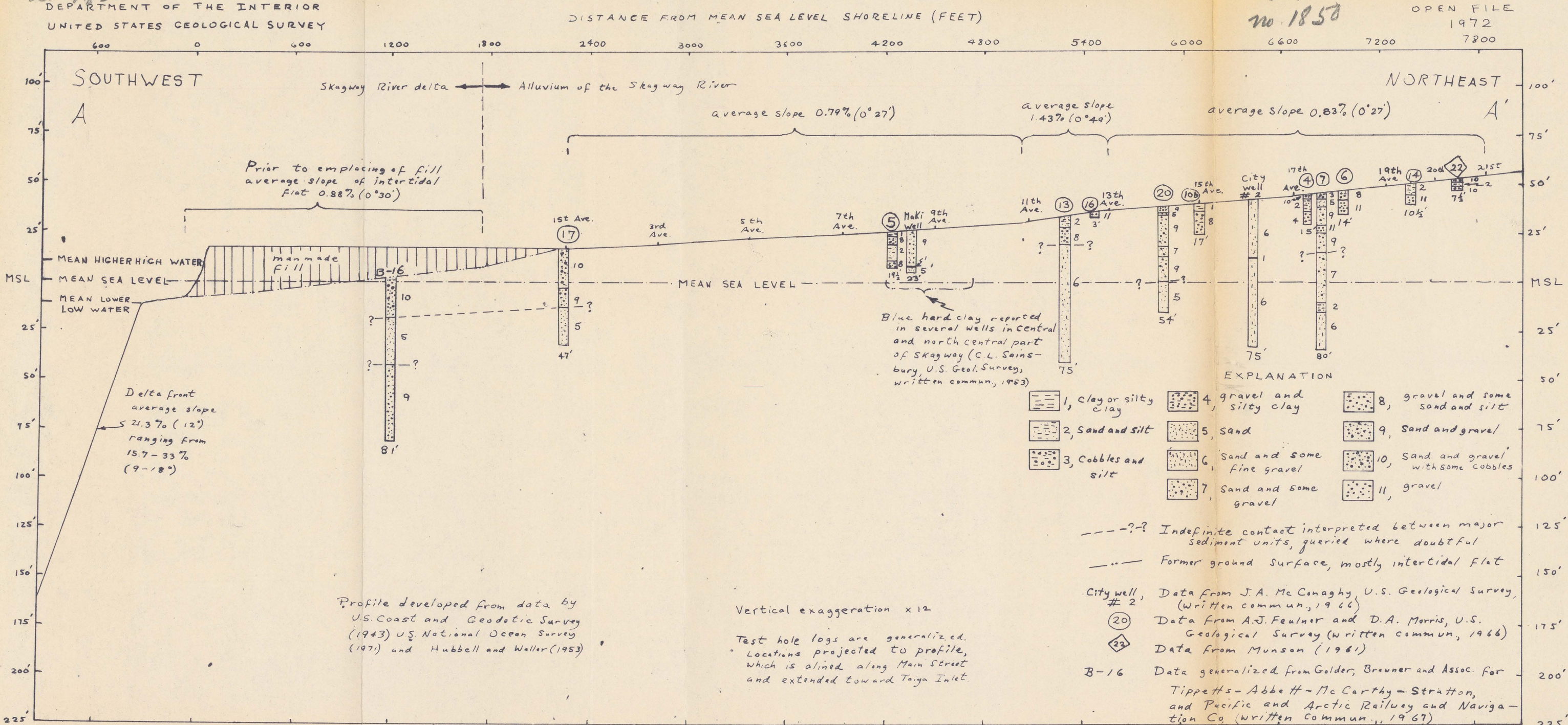
Figure 7.— Profile A-A' along part of lower Skagway valley and Skagway River delta and data from selected test holes. See figures 4 and 6 for locations.
