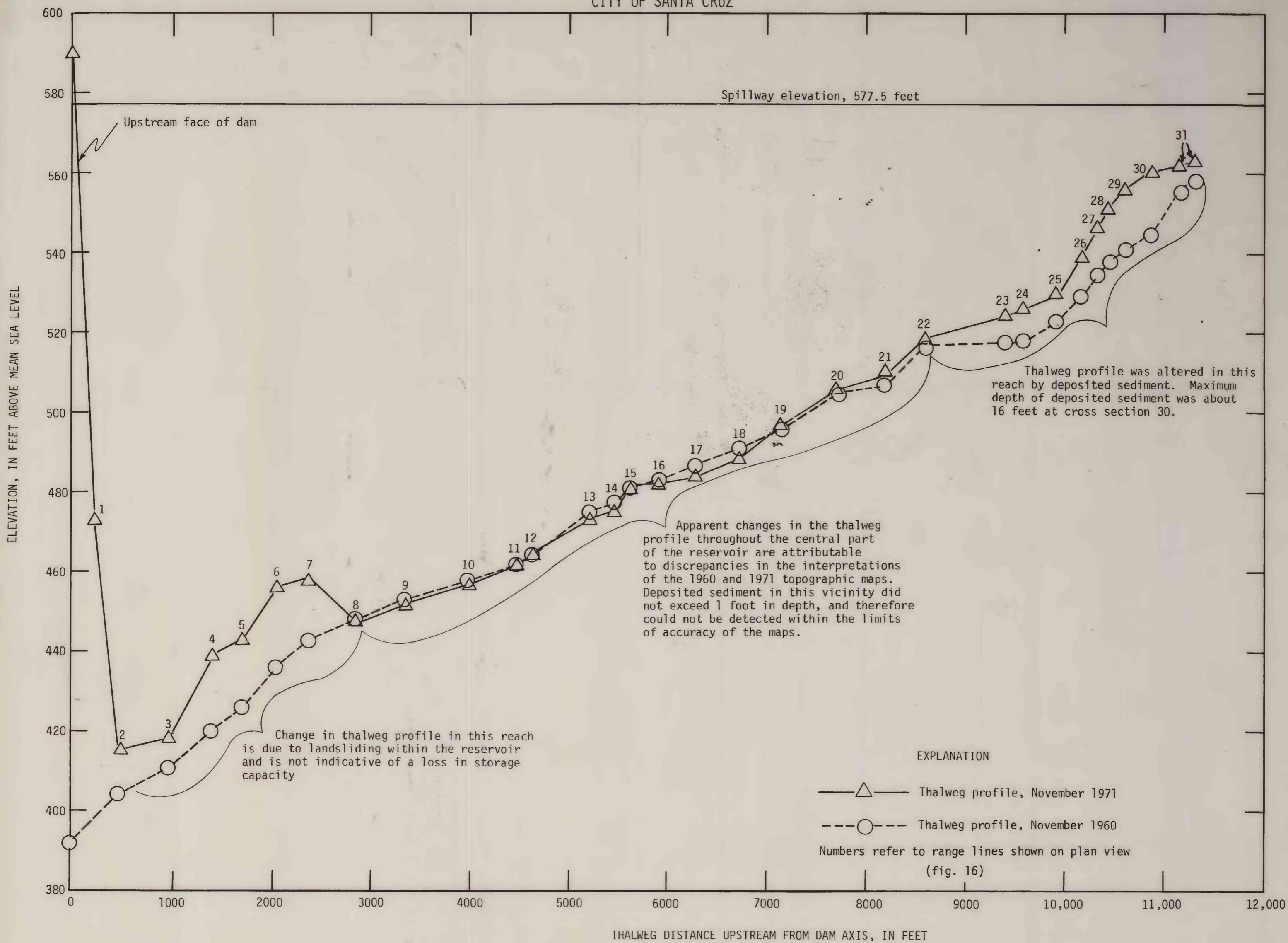
FIGURE 15.--THALWEG PROFILES OF LOCH LOMOND SHOWING LOCATION OF CROSS SECTIONS USED IN 1971 RESERVOIR SURVEY
