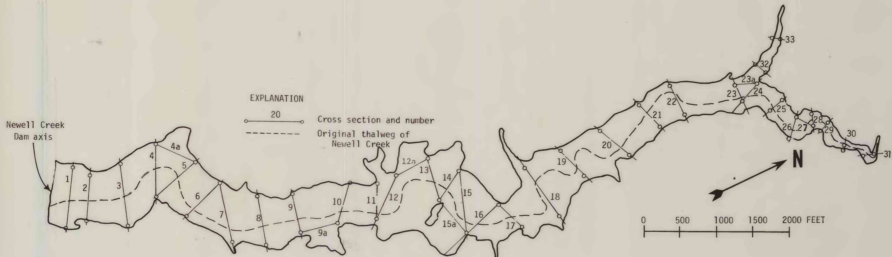
FIGURE 16.--PLAN VIEW OF LOCH LOMOND SHOWING LOCATION OF CROSS SECTIONS USED IN 1971 RESERVOIR SURVEY
