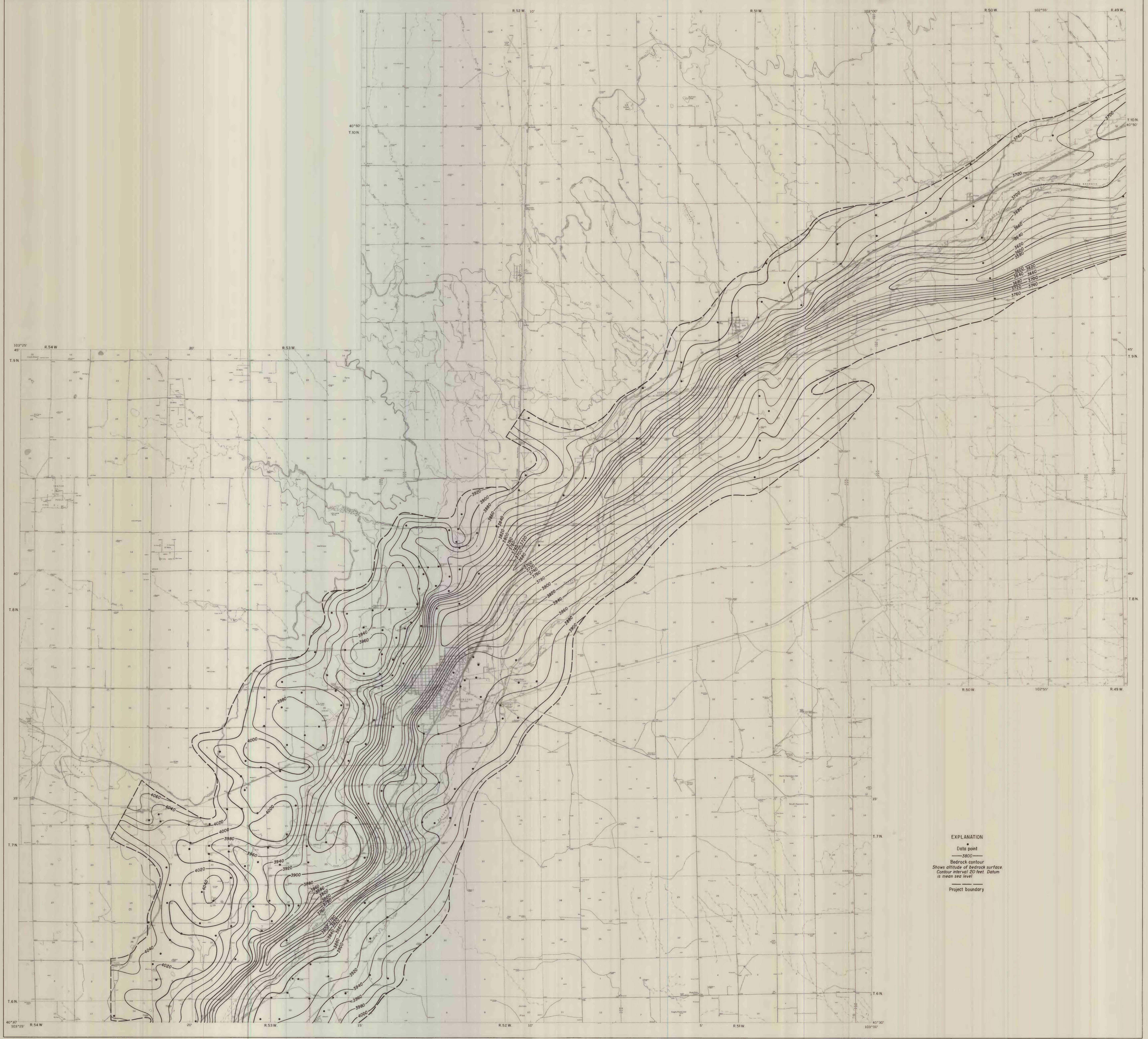
MAP SHOWING BEDROCK CONFIGURATION BENEATH THE VALLEY-FILL AQUIFER IN THE STERLING REACH OF THE SOUTH PLATTE RIVER VALLEY, COLORADO By Paul A. Schneider, Jr., and Warren E. Hofstra 1972
