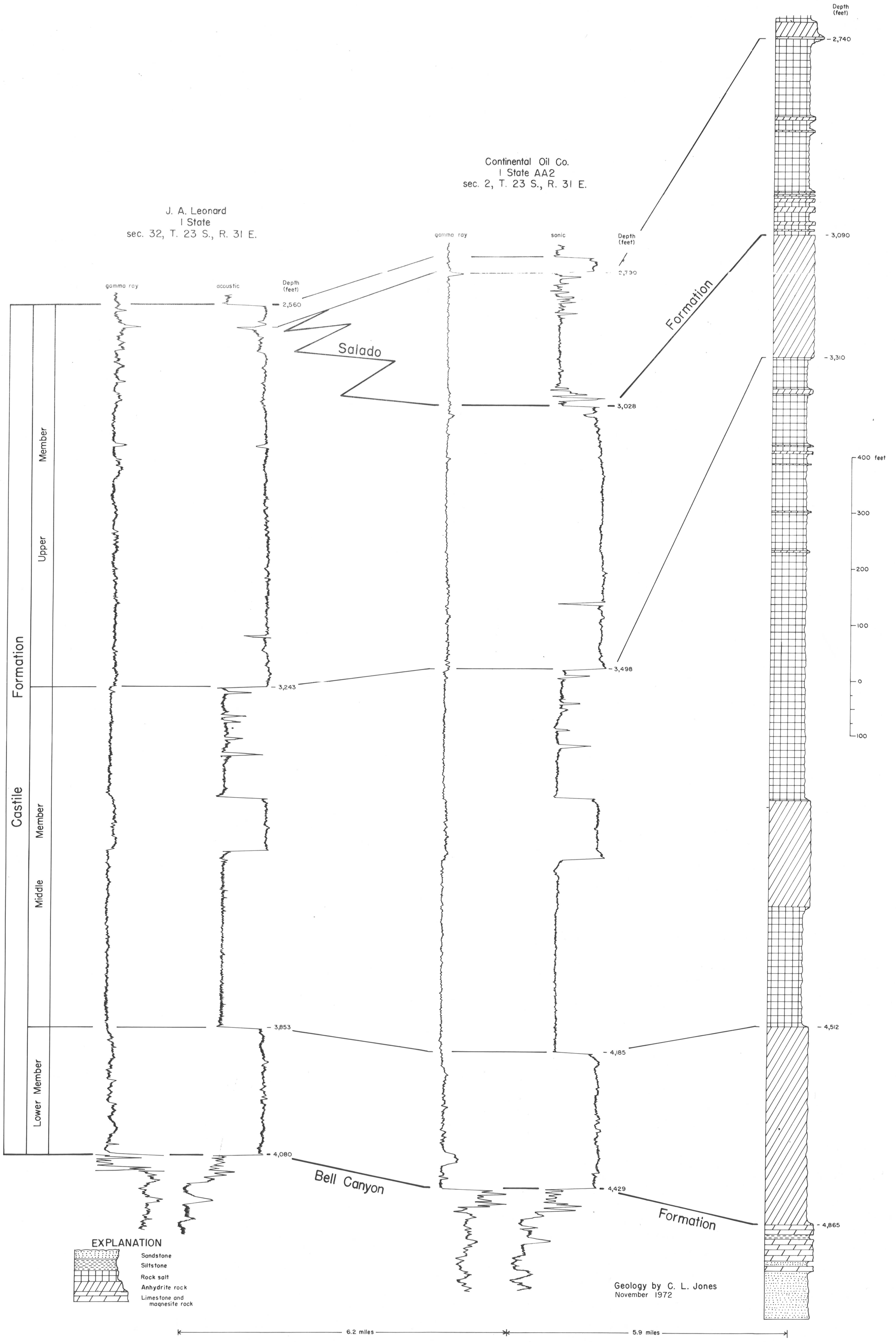
SUBSURFACE SECTIONS OF THE CASTILE FORMATION LOS MEDAÑOS AREA, EDDY AND LEA COUNTIES, NEW MEXICO
