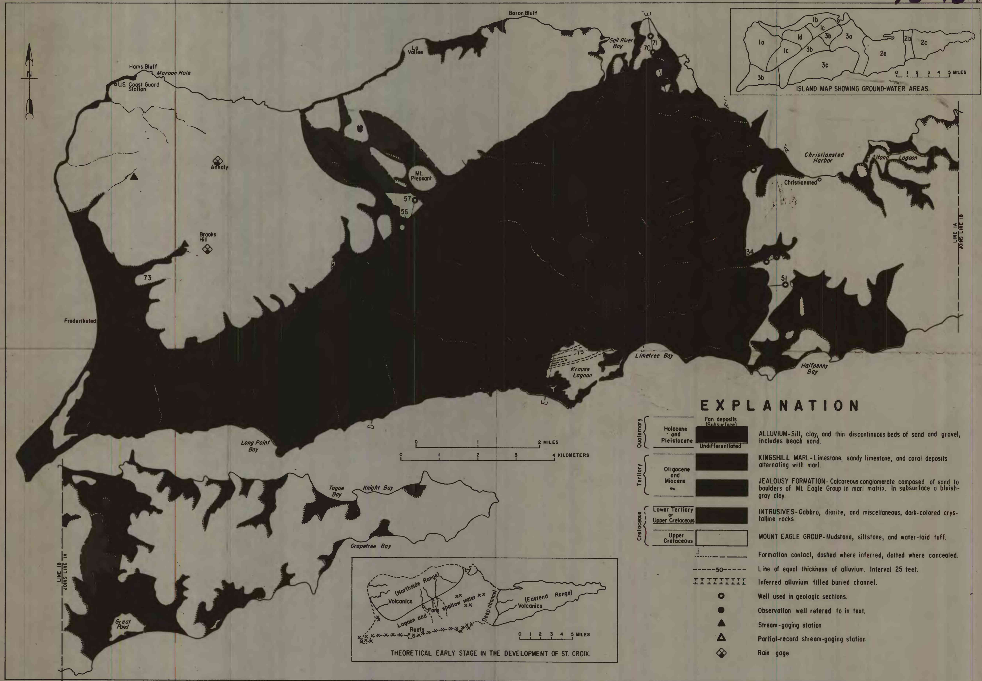
FIGURE 5a.--GENERALIZED GEOLOGY, LOCATION OF STREAM-GAGING SITES, OBSERVATION WELLS, AND GROUND-WATER AREAS.
