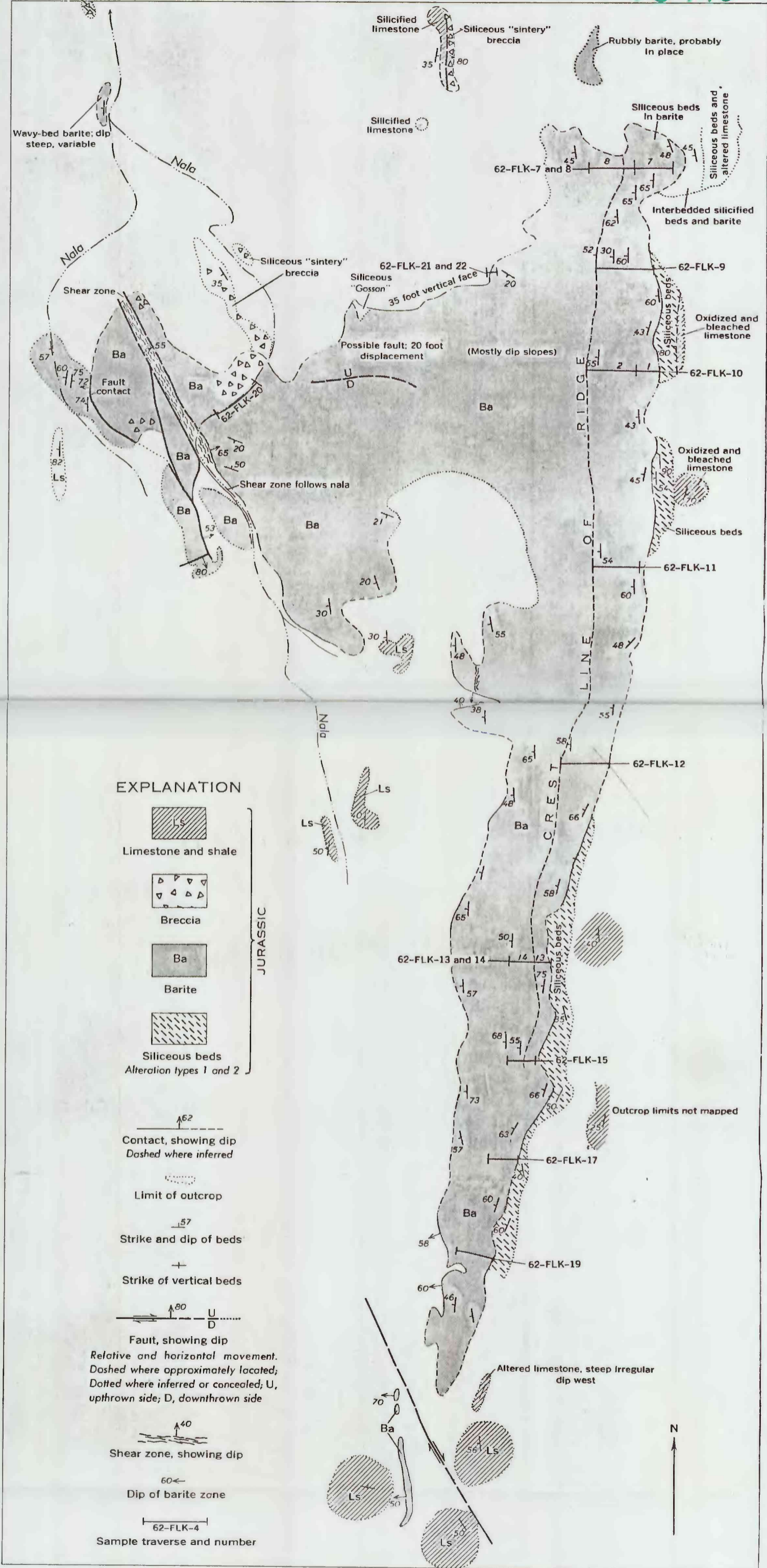
Figure 9—Sketch map of the principal Gunga barite deposit.
