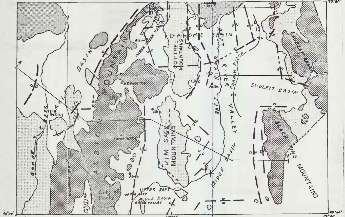
Figure 4. Map showing major structures inferred from gravity and magnetic anomalies in Albion Mountains and adjoining areas.
