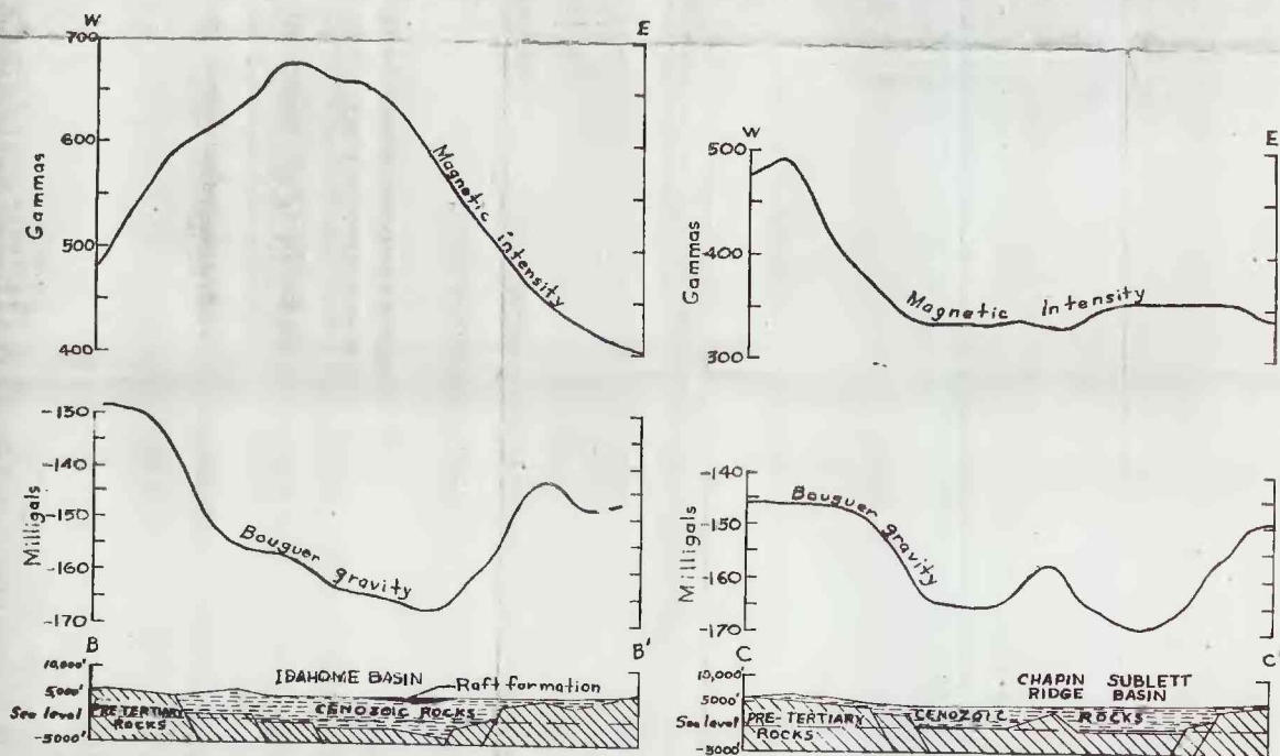
Figure 5. Section showing interpretation of gravity and magnetic data along profiles.
