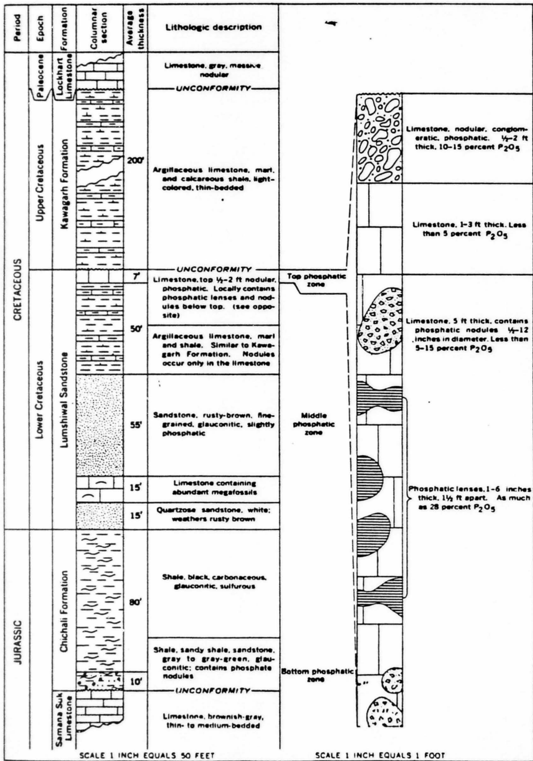
Figure 2.—Stratigraphic section of phosphatic rock in the Nizampur area
