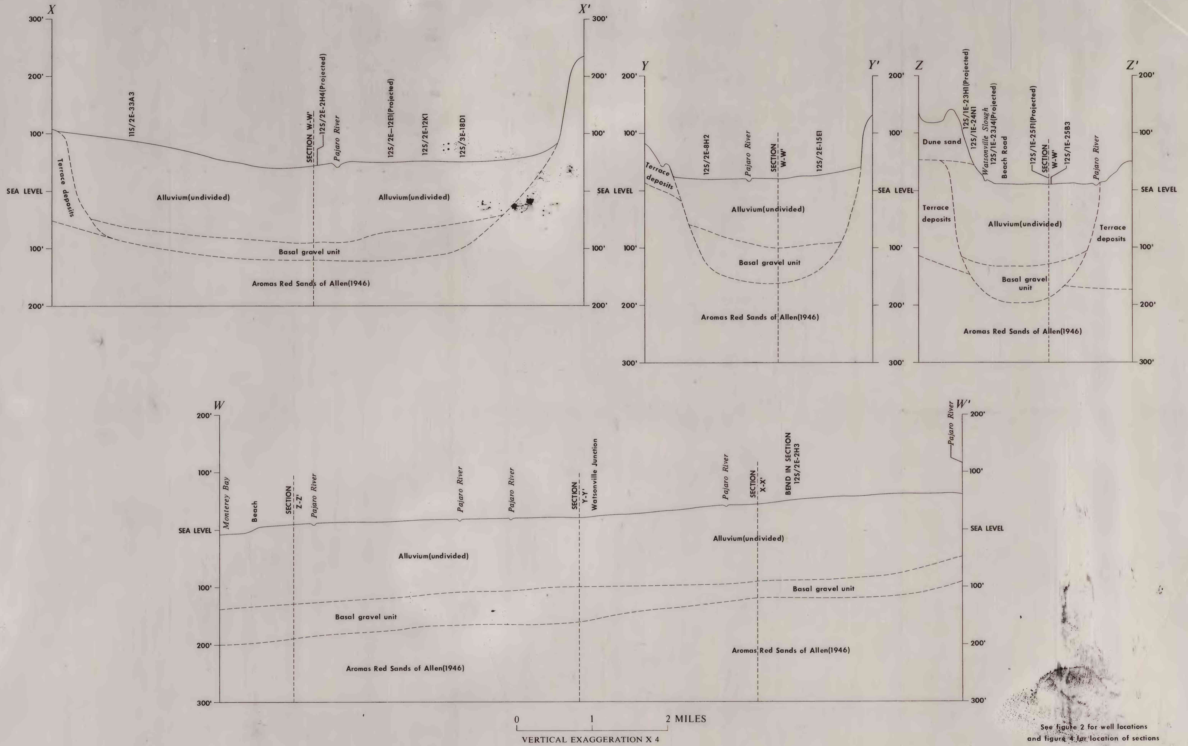
GEOLOGIC SECTIONS OF THE PAJARO VALLEY AREA, SANTA CRUZ AND MONTEREY COUNTIES, CALIFORNIA SHOWING BASAL GRAVEL UNIT IN ALLUVIUM
