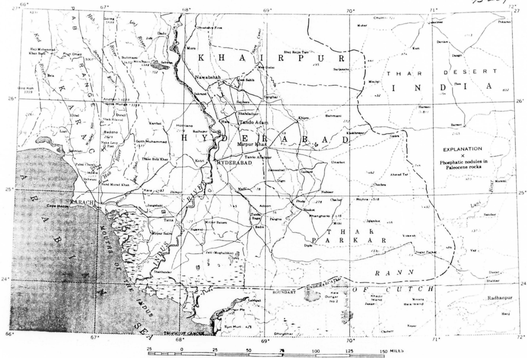
Figure 2.—Base sheet B, Pakistan, showing the location of phosphatic nodules found in rocks of Paleocene age in the southern part of the Pab Range
