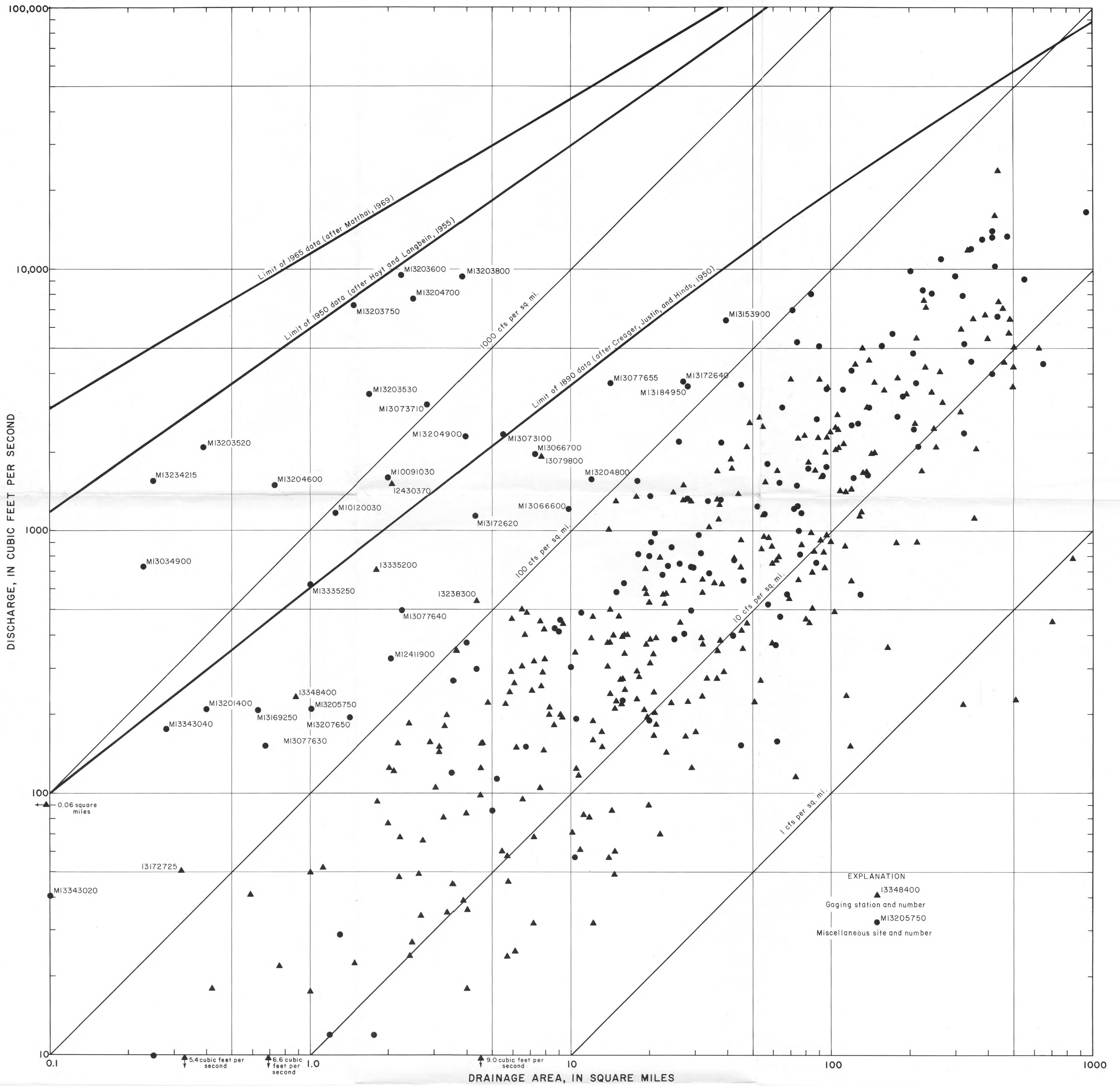
FIGURE 3.--MAXIMUM DISCHARGES IN RELATION TO DRAINAGE AREA.
