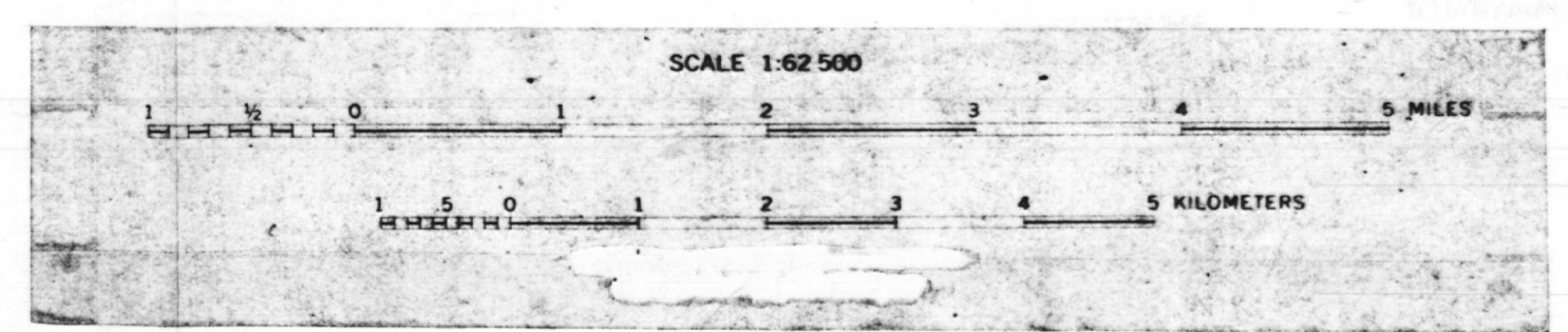
AEROMAGNETIC MAP OF NORTHERN FREDERICK COUNTY, MARYLAND AND PARTS OF ADJACENT COUNTIES IN MARYLAND AND PENNSYLVANIA 1973
