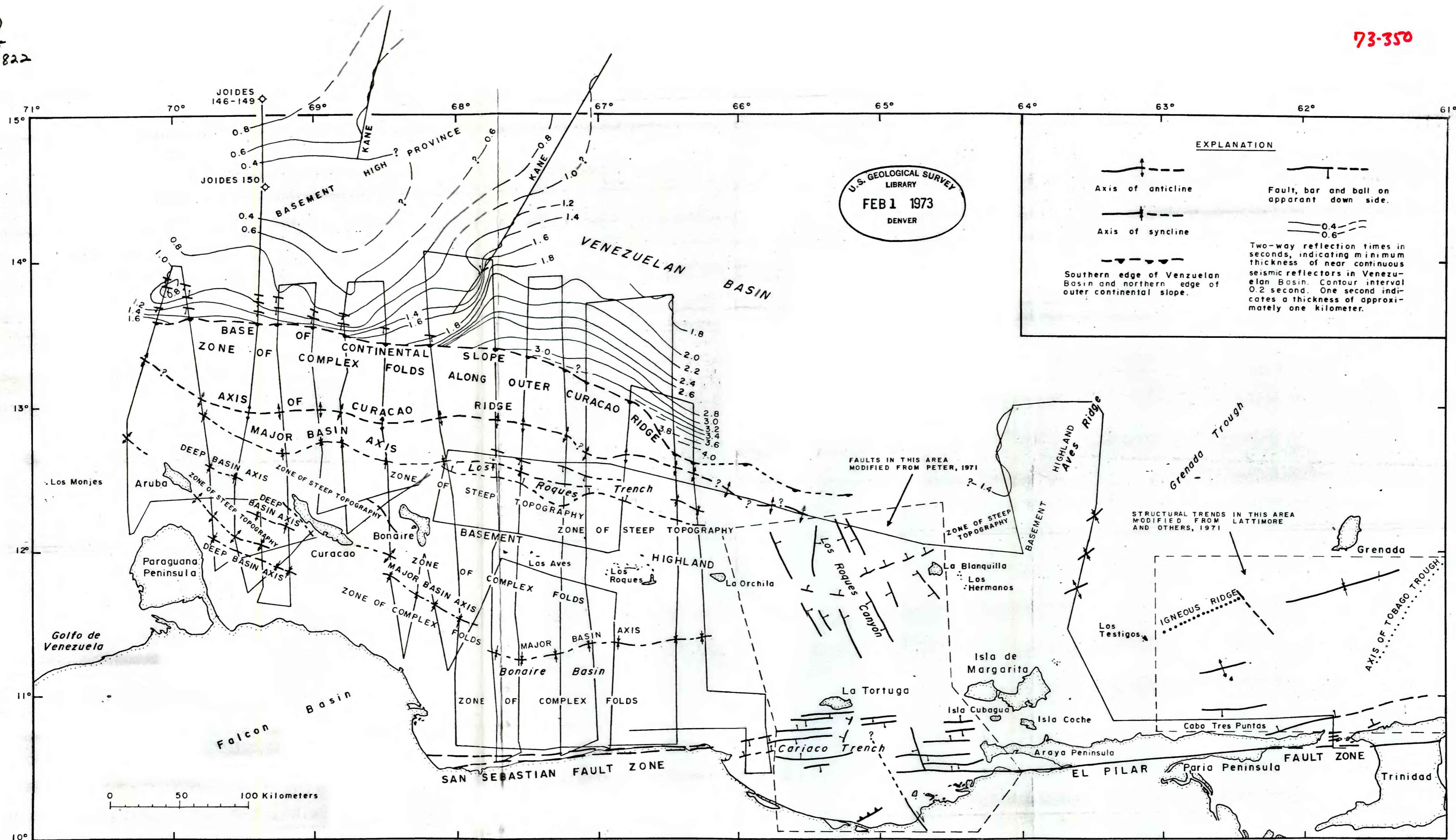
FIGURE 5-- SIMPLIFIED TECTONIC MAP, VENEZUELAN BORDERLAND
