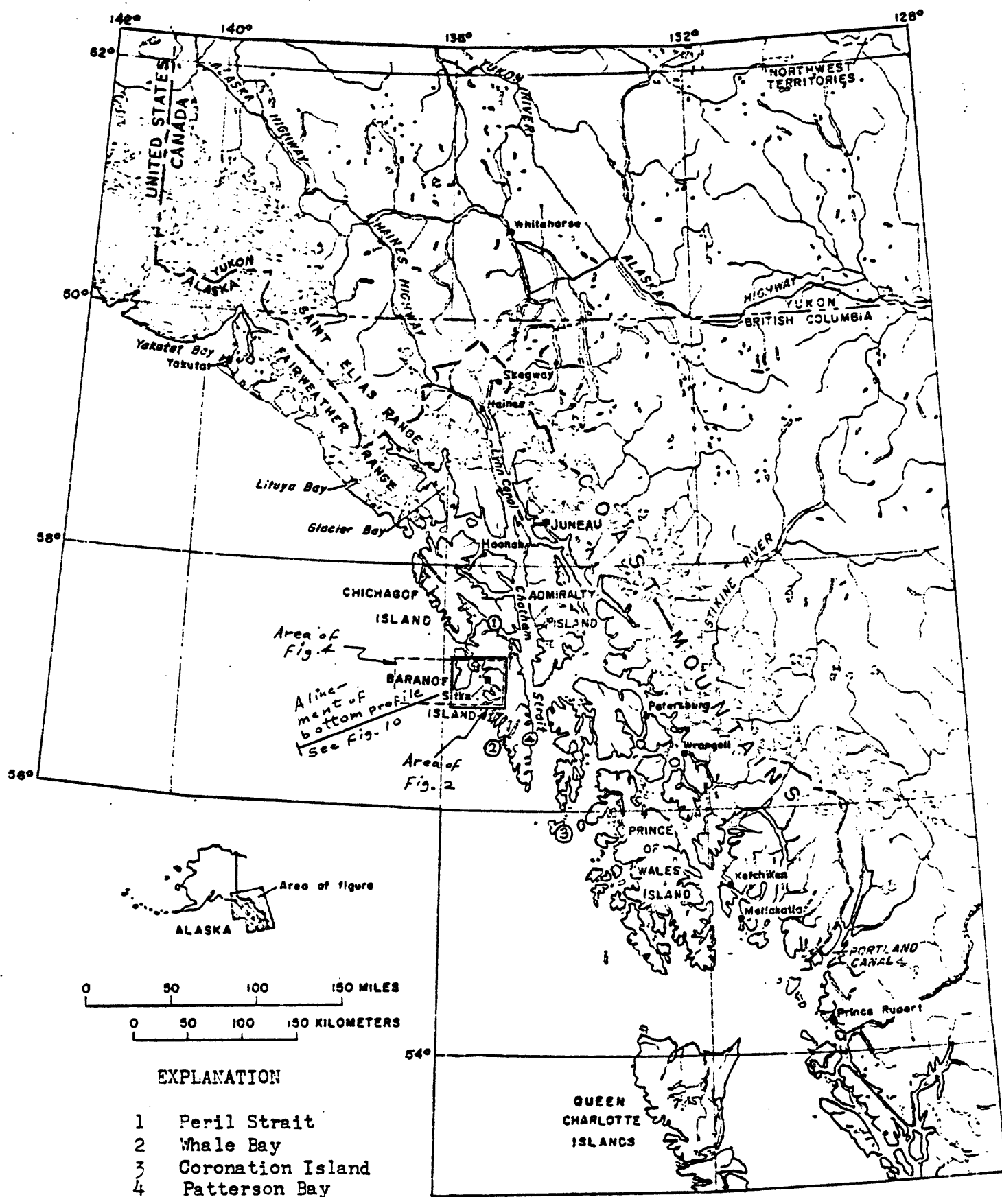
Figure 1.--Southeastern Alaska and adjacent part of Canada showing selected geographic features.
