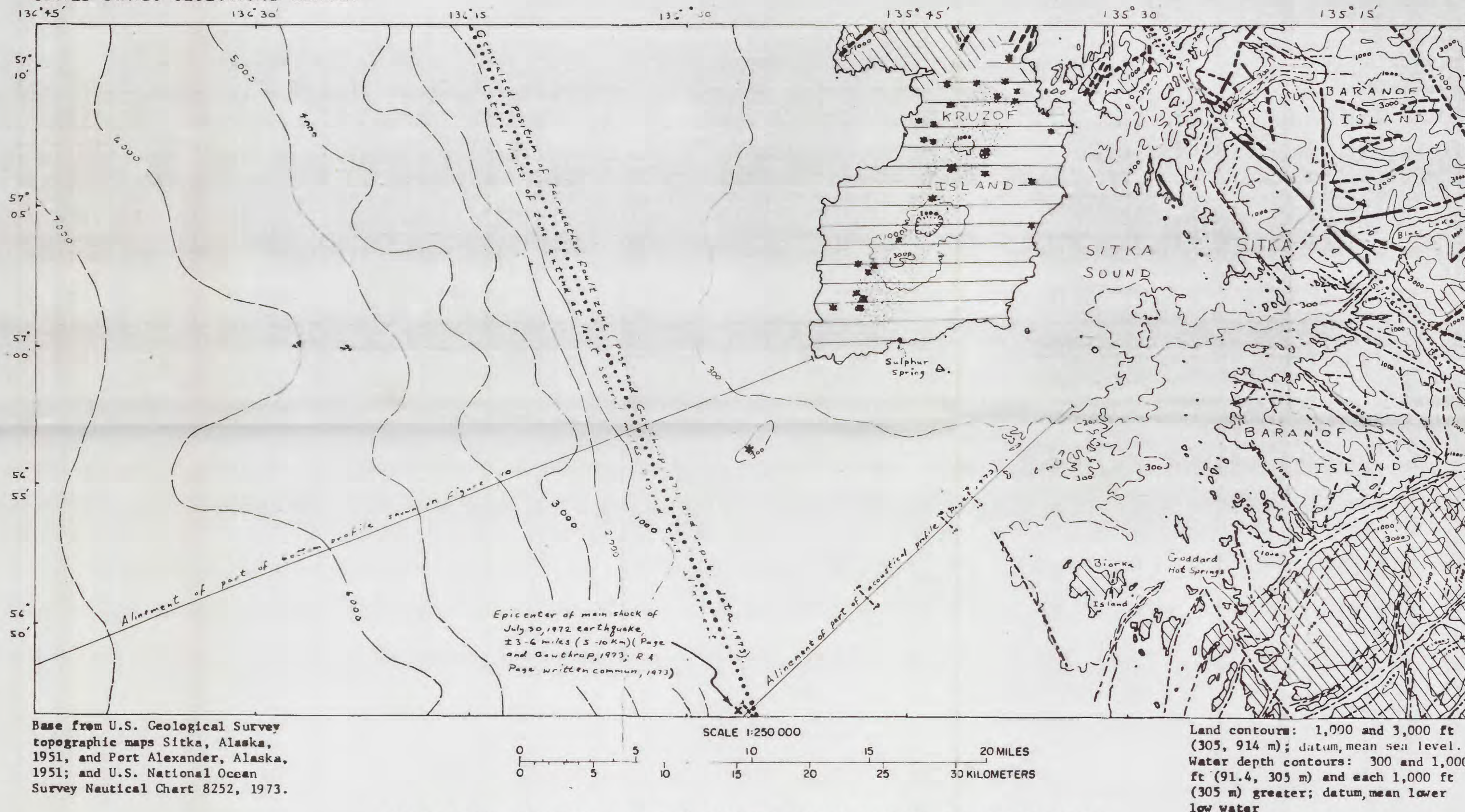
FIGURE 4.--MAP SHOWING FAULTS AND OTHER LINEAMENTS, BEDROCK TYPES, AND OFFSHORE WATER DEPTHS, SITKA AREA, ALASKA, AND PART OF CONTINENTAL MARGIN
