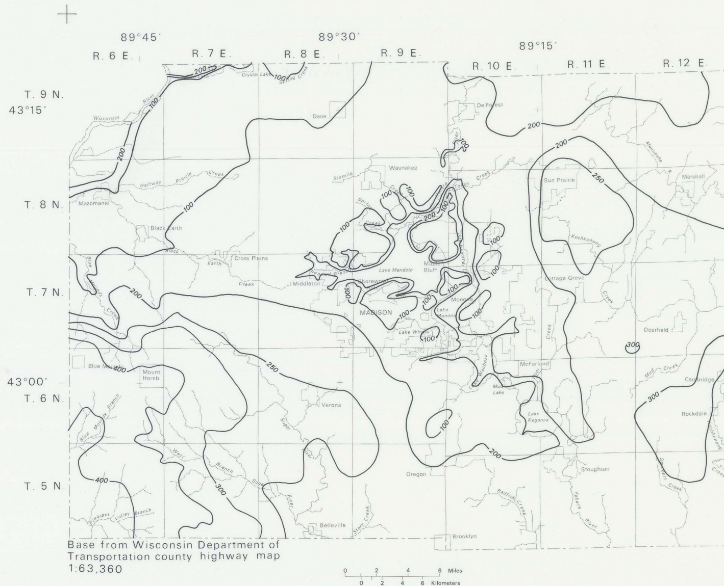
Figure 10. Saturated thickness of the upper aquifer before development.
