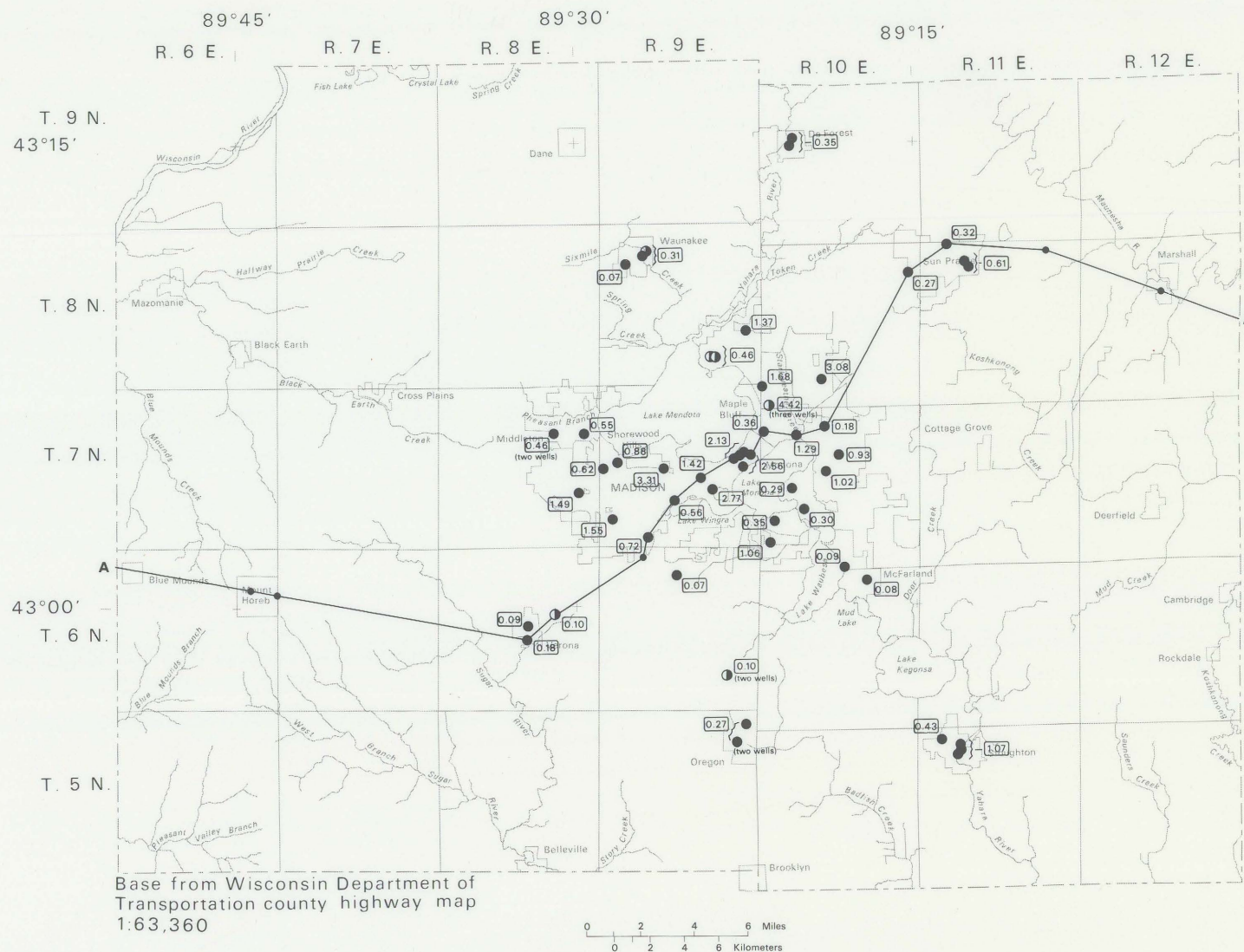
Figure 12. Pumpage from the sandstone aquifer during 1970.
