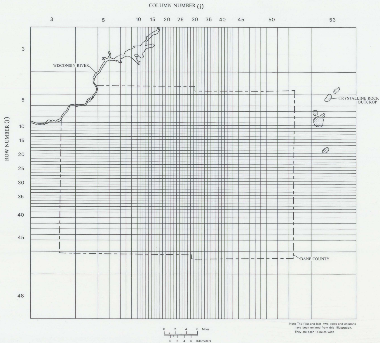
15 Figure 13. Finite-difference grid used for modeling the sandstone aquifer.
