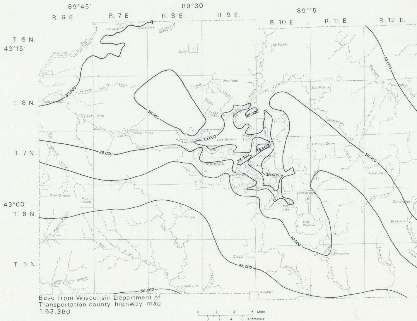
Figure 16. Transmissivity in the sandstone aquifer.
