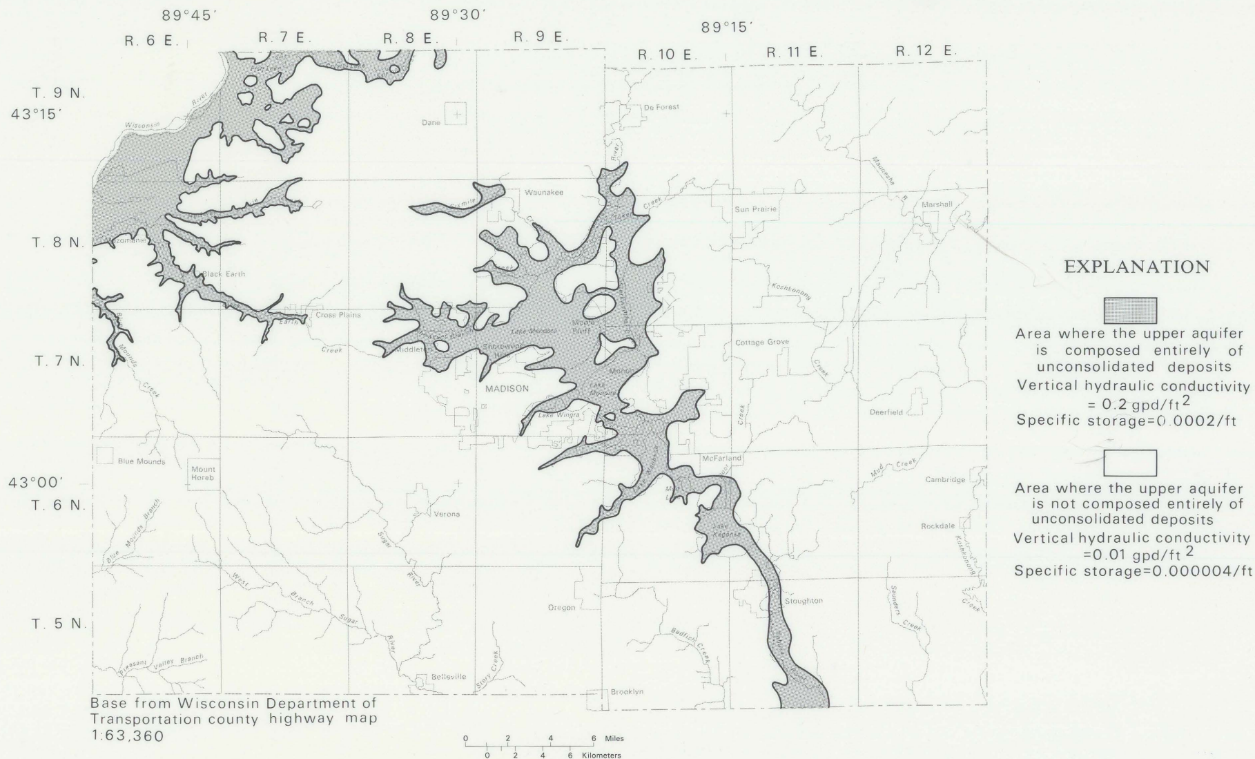
Figure 18. Vertical hydraulic conductivity and specific storage in the upper aquifer.
