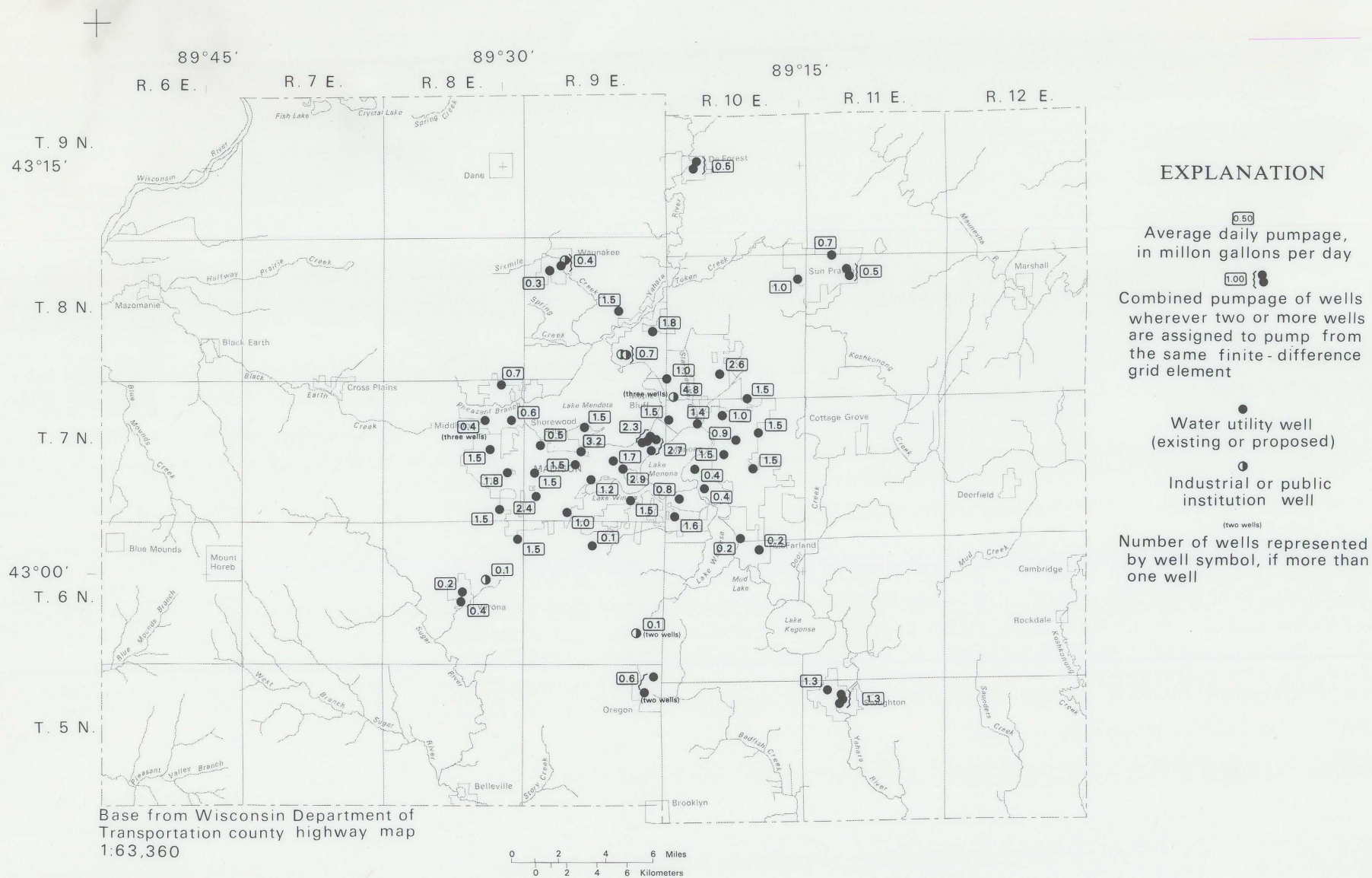
Figure 21. Estimated pumpage from the sandstone aquifer by 1990.
