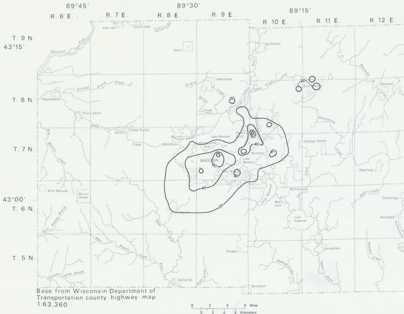
Figure 22. Computer drawdowns in the sandstone aquifer by 1980.
