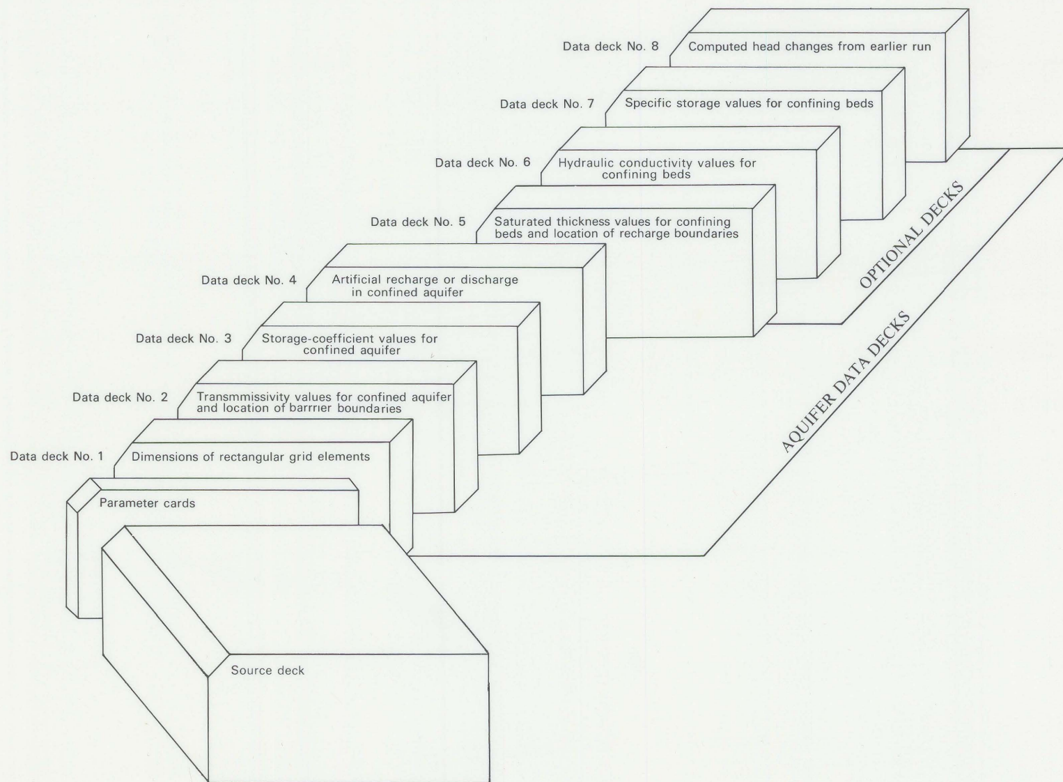
Figure 4. Assembled digital computer program.
