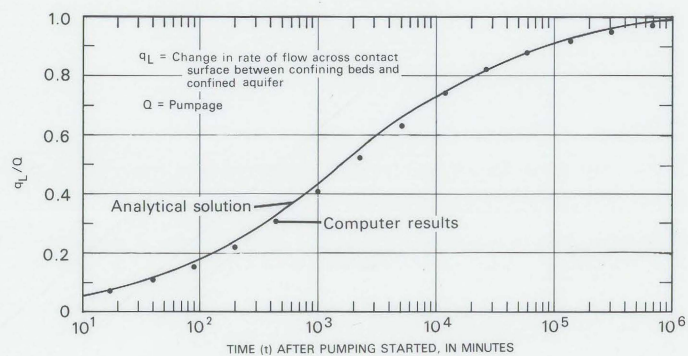
Time-leakage curve through leaky confining beds
