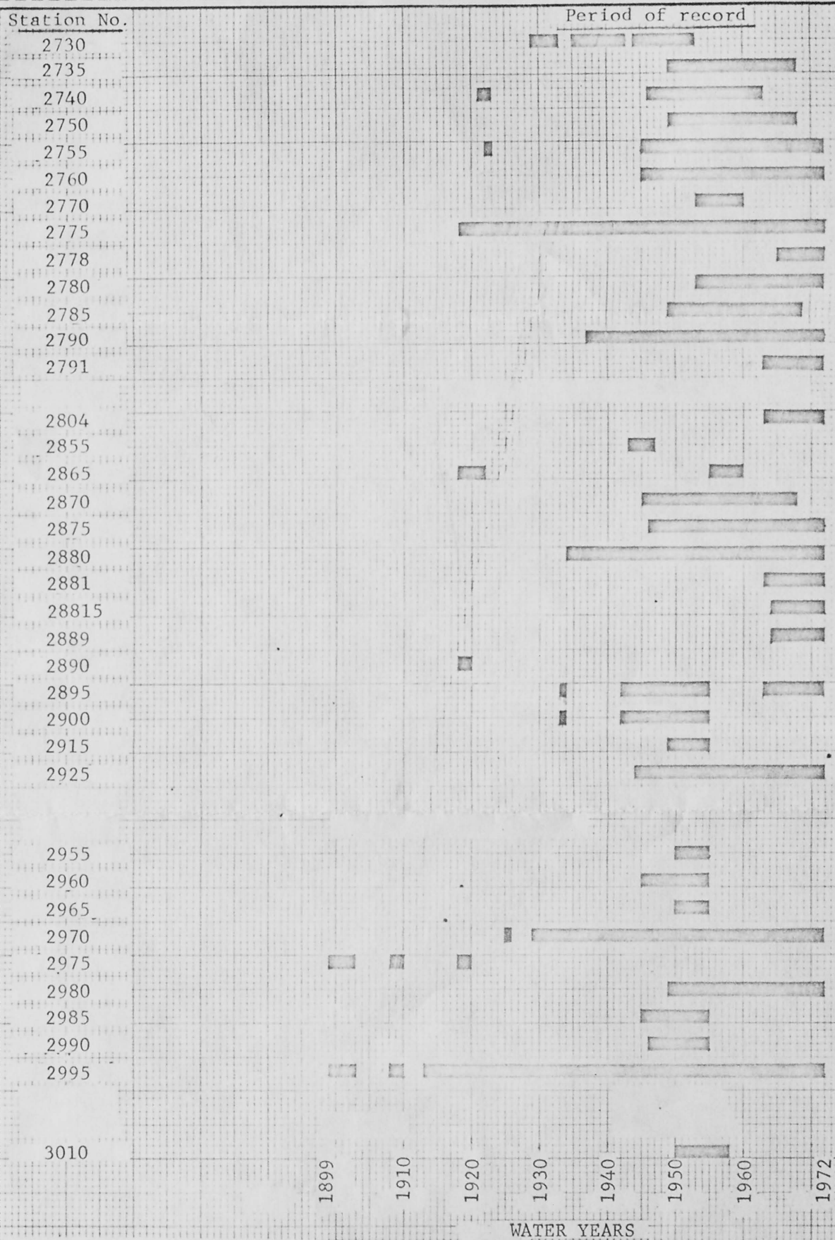
Figure 2. Period of record of selected gaging stations in the Duchesne River basin.
