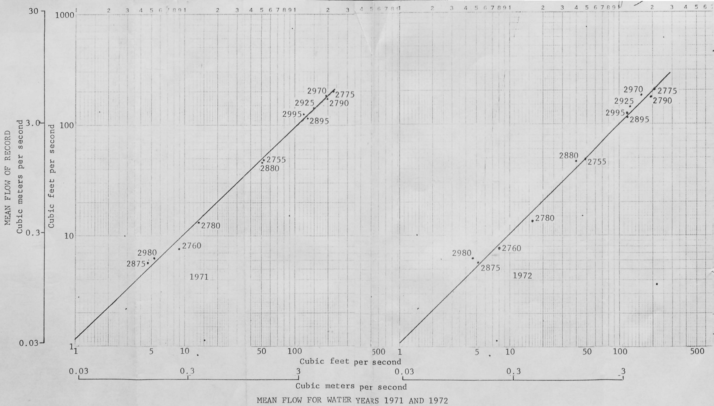
Figure 4.--Relation of mean flow for the 1971 and 1972 water years to mean flow of record at selected gaging stations.
