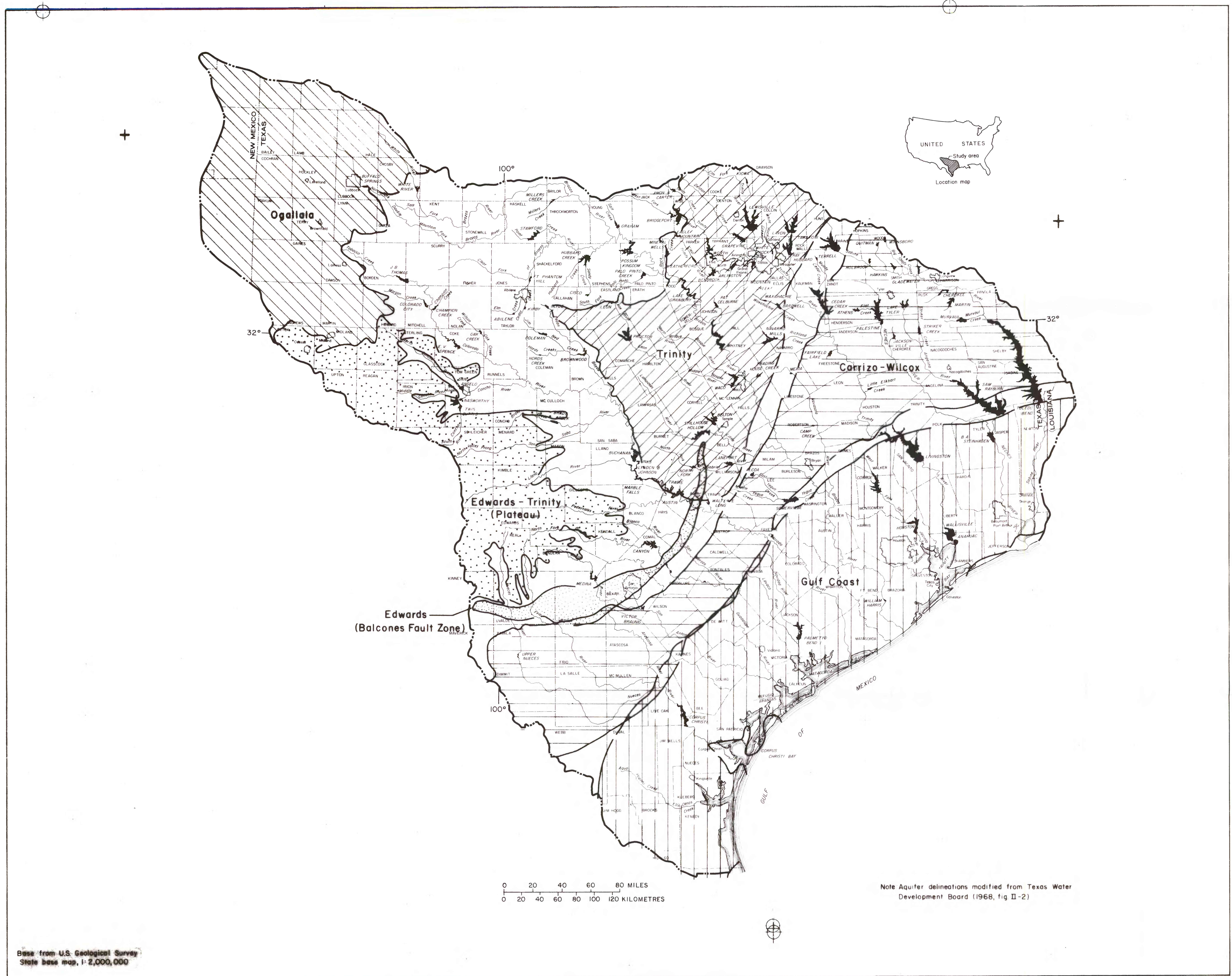
FIGURE 5.-Location and extent of aquifers (Sheet 2 of 2)
