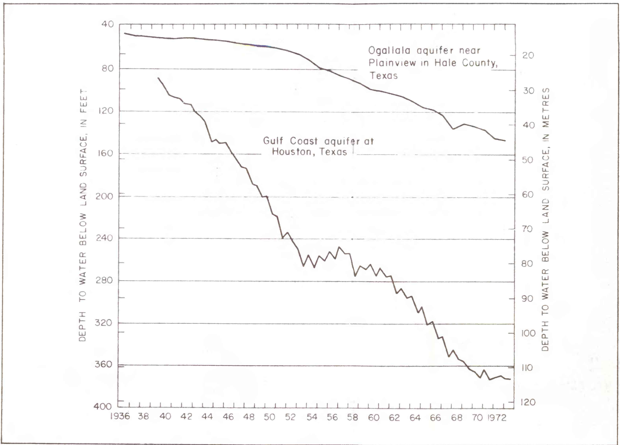
FIGURE 8.-Water-level declines in the Ogallala aquifer near Plainview, Texas, and in the Gulf Coast aquifer at Houston, Texas
