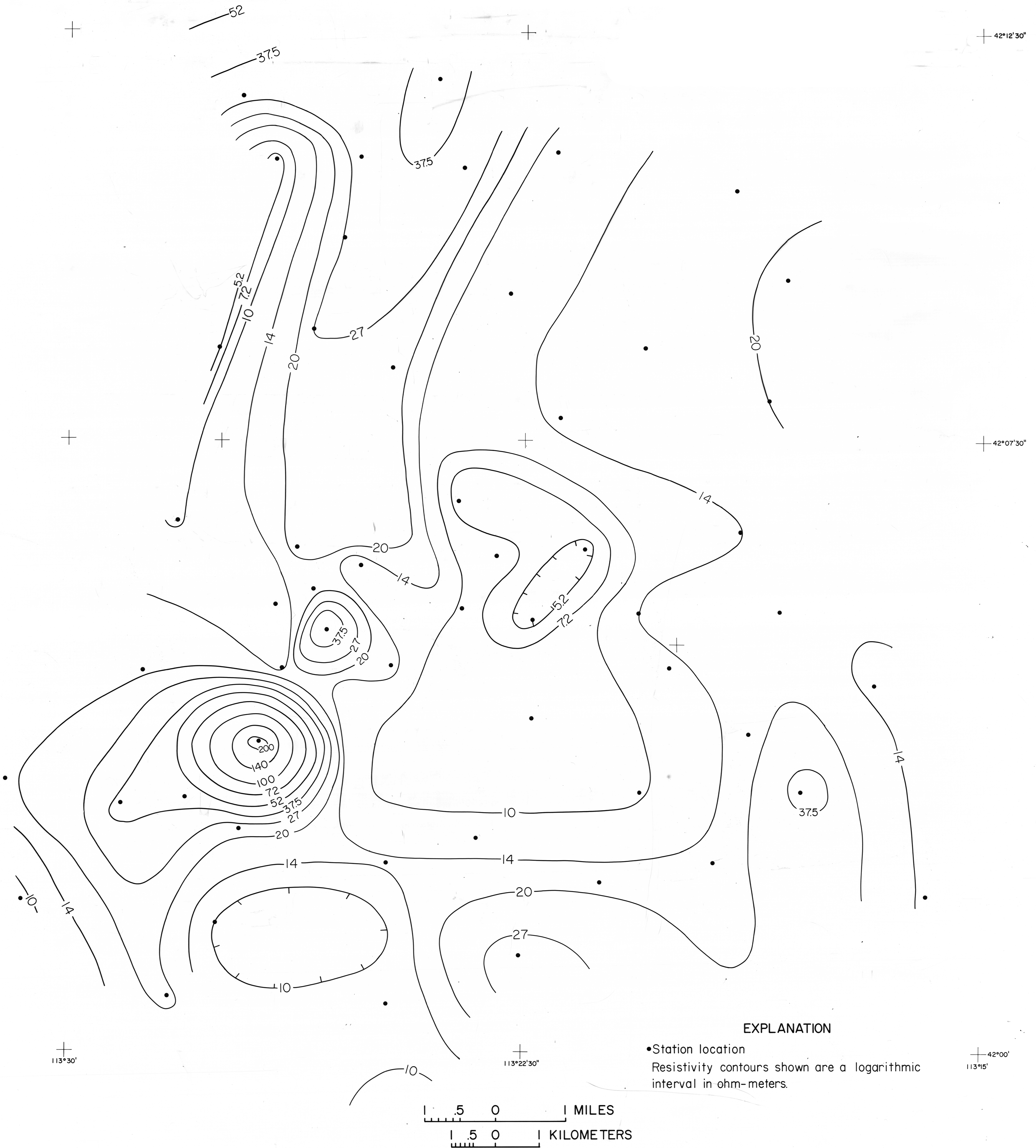
26 HERTZ; TELLURIC LINE EAST-WEST AUDIO-MAGNETOTELLURIC APPARENT RESISTIVITY MAPS, SOUTHERN RAFT RIVER AREA, CASSIA COUNTY, IDAHO 1974 BY D.B. HOOVER
