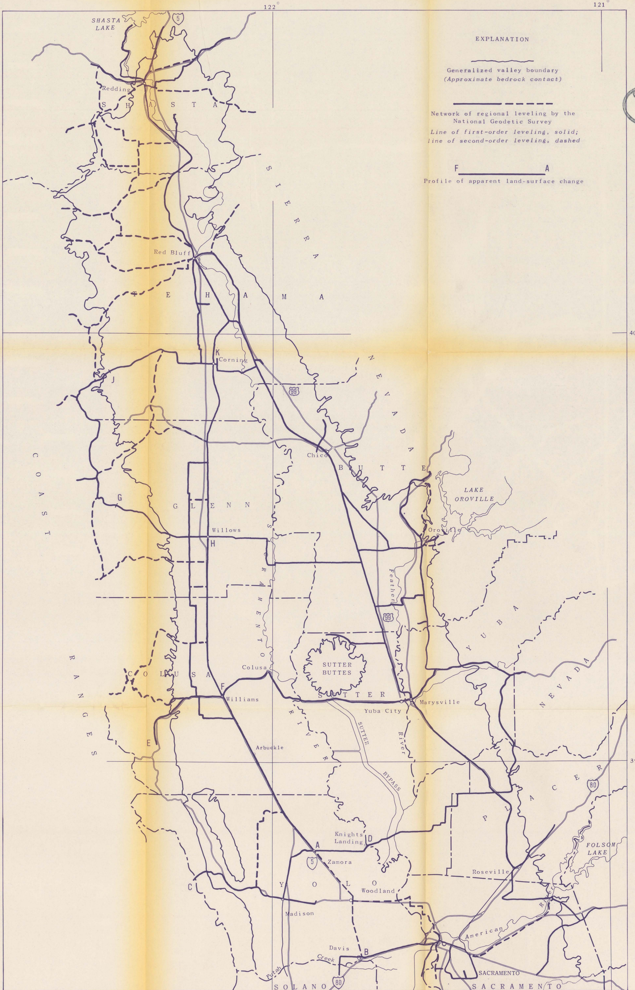
FIGURE 1.—Network of regional leveling by the National Geodetic Survey, Sacramento Valley, California
