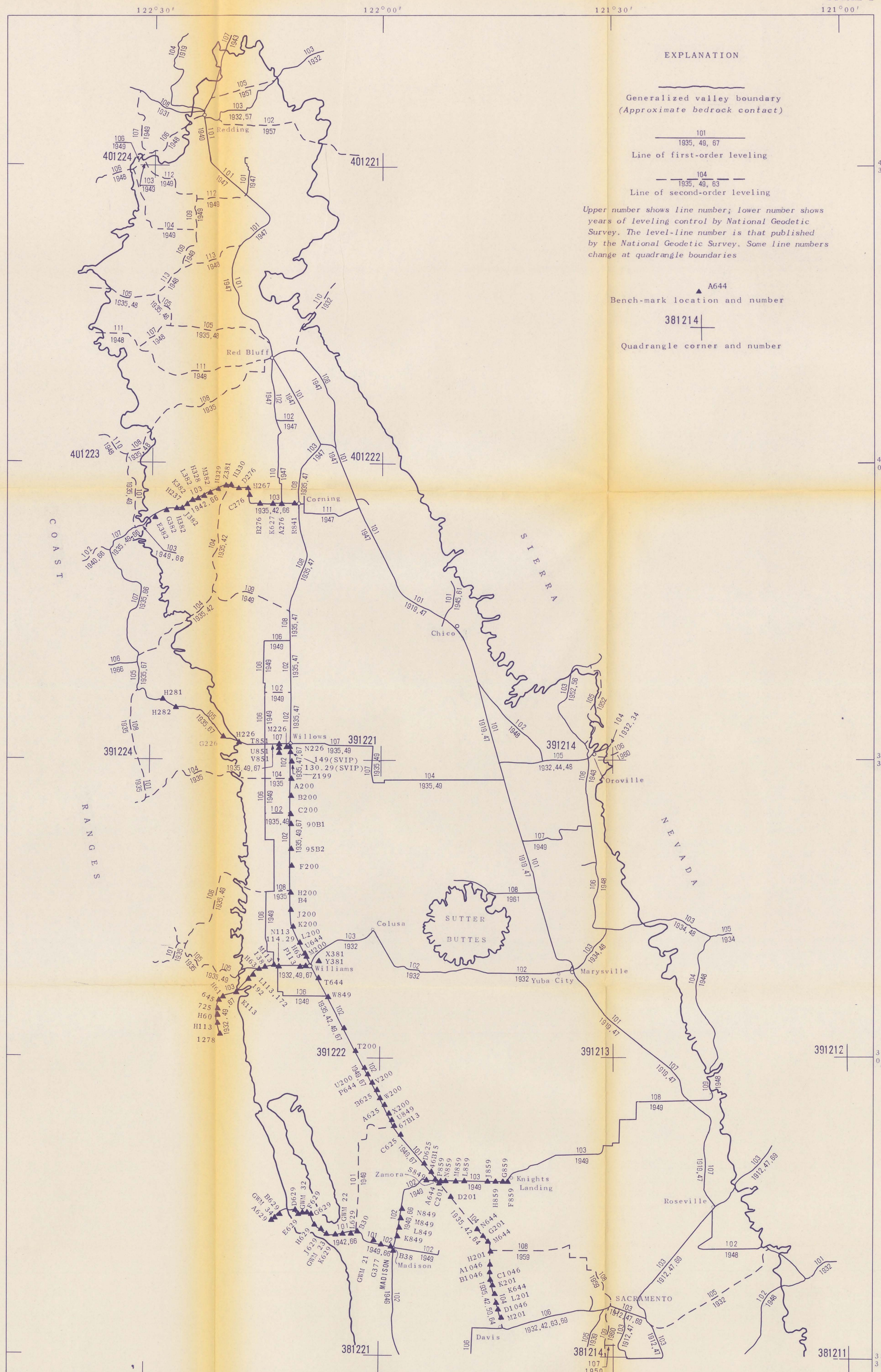
FIGURE 2.—Years of leveling by the National Geodetic Survey and location of bench marks for which repeated leveling indicates change in land-surface elevation, Sacramento Valley, California
