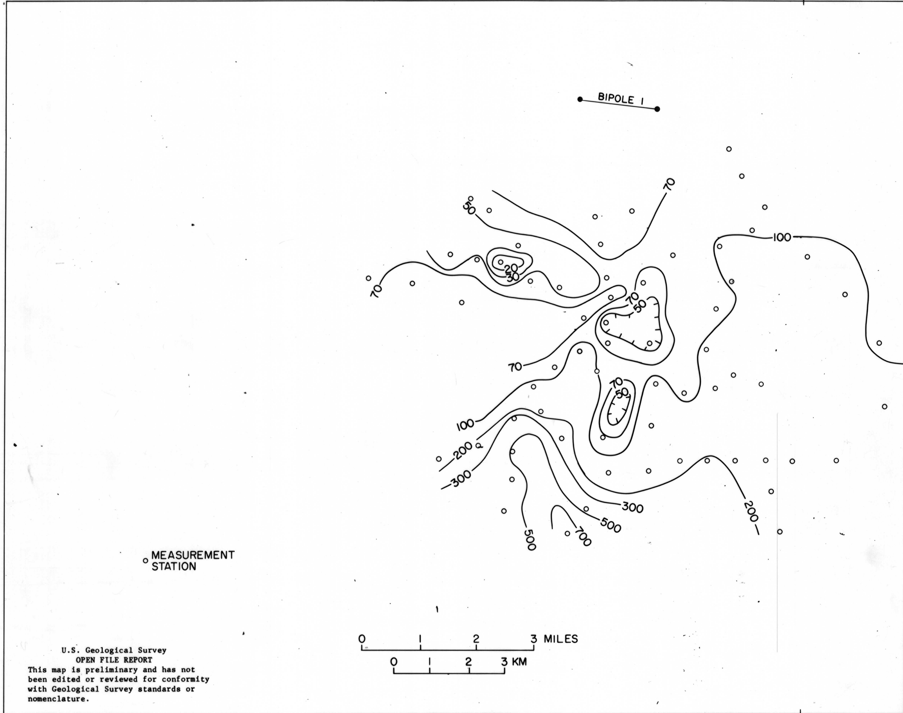
Plate 3.--Total-field resistivity map for bipole 1, Long Valley caldera, California.
