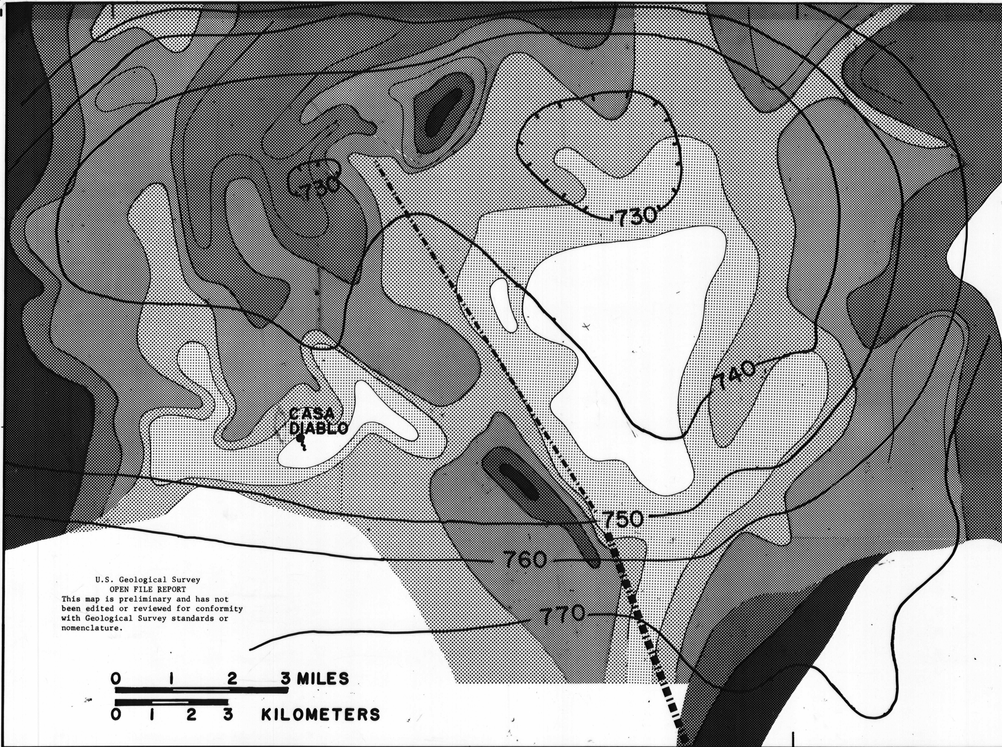
Plate 7.--Bouguer gravity map of Long Valley caldera, California, superimposed on composite total-field resistivity map.
