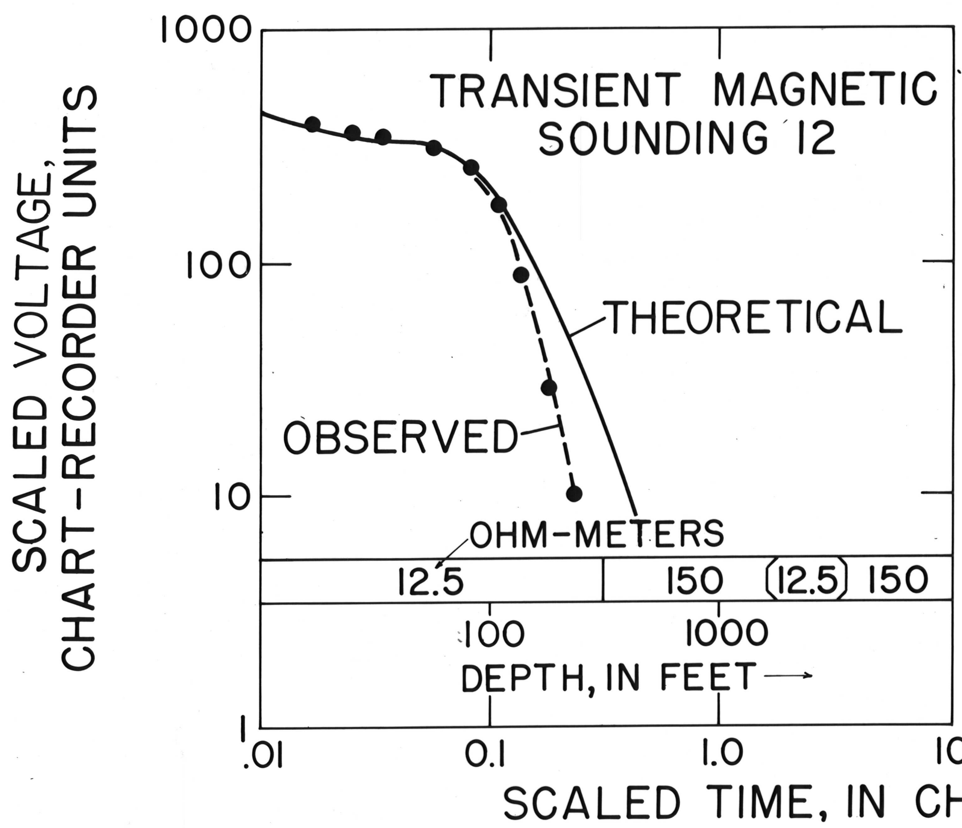
Plate 13.--Sounding curves and interpretations for soundings which detected the deep conductor, Long Valley caldera, California.
