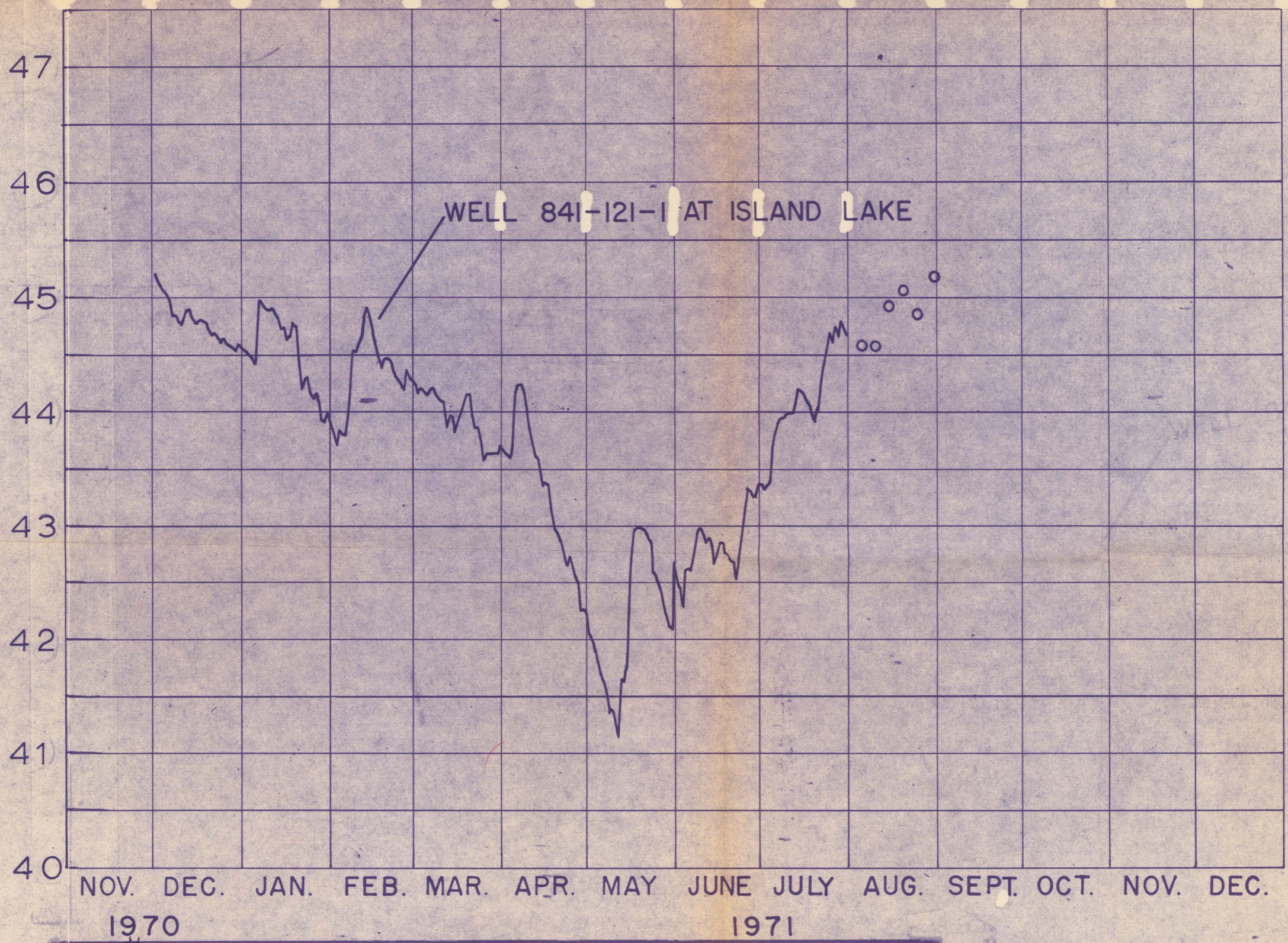
Figure 1.--Hydrographs for Island Lake and well 841-121-1.
