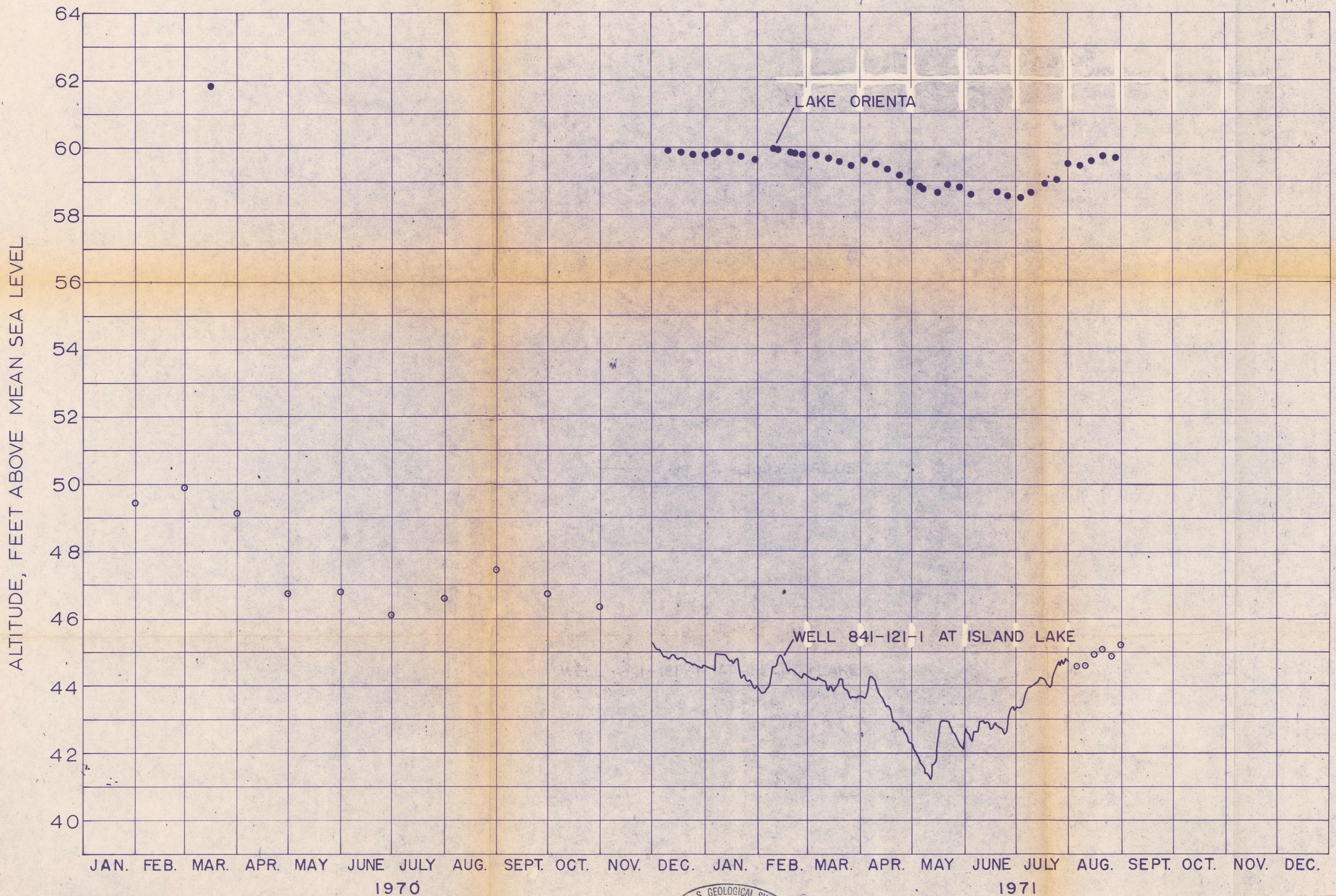
12 Figure 12--Hydrographs for Lake Orienta and well 841-121-1.
