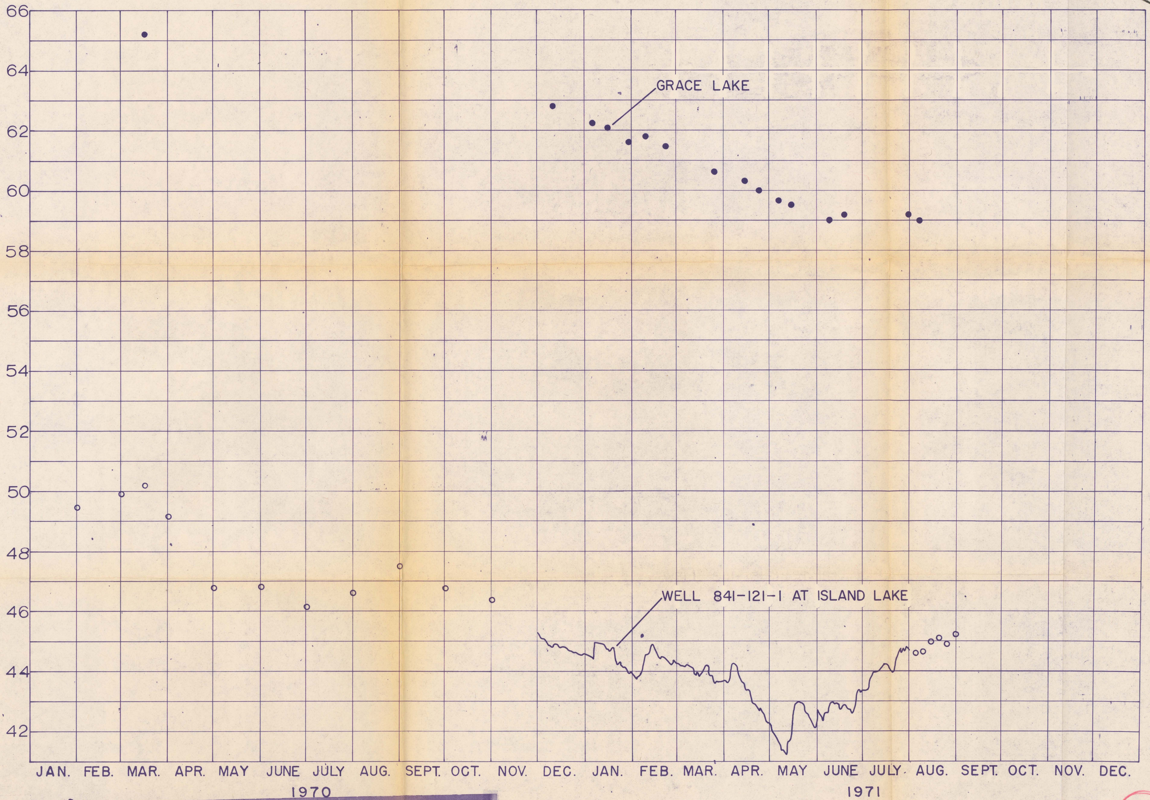
13 Figure 13.--Hydrographs for Grace Lake and well 841-121-1.
