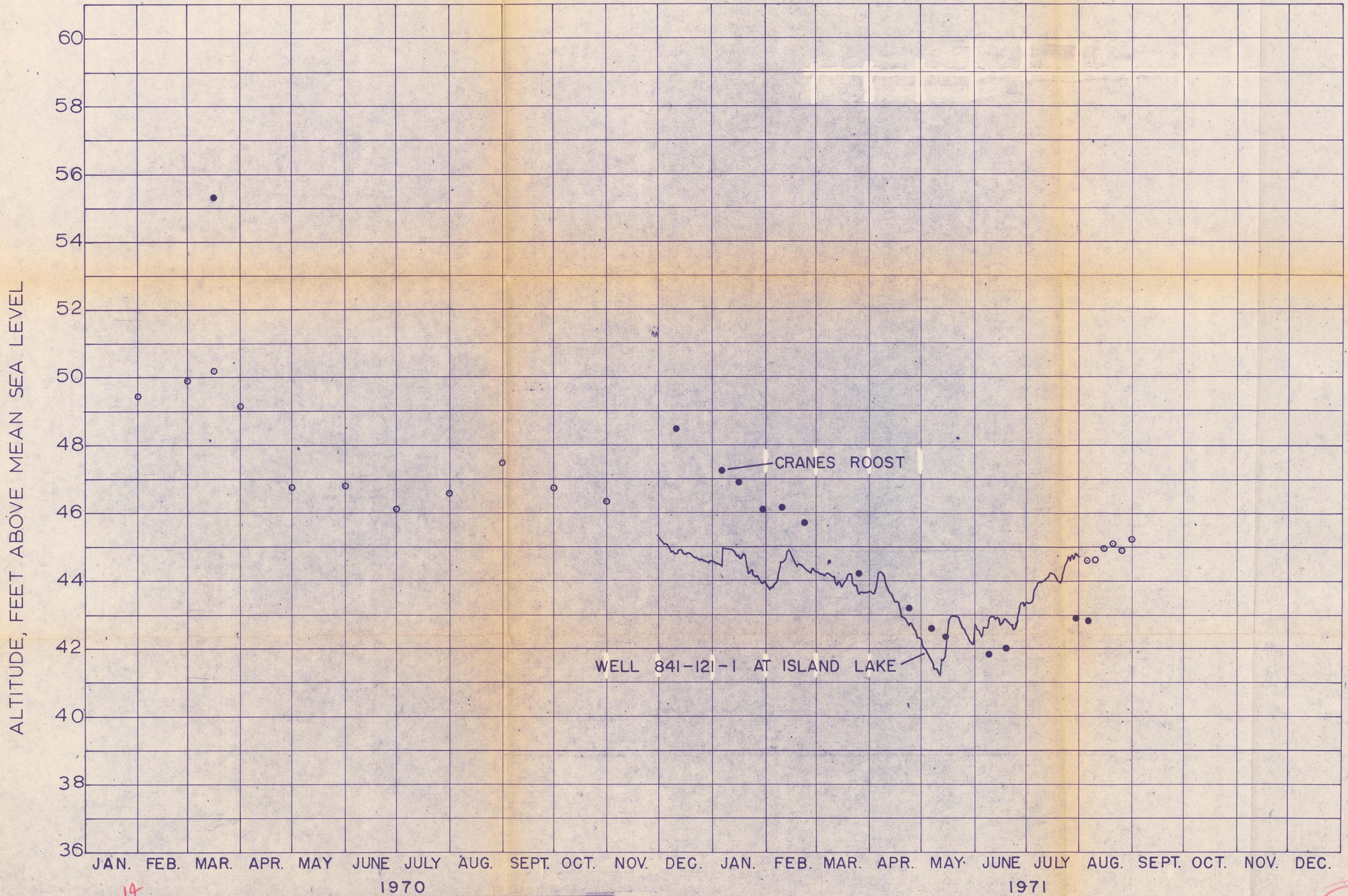
14 Figure 14--Hydrographs for Cranes Roost and well 841-121-1.
