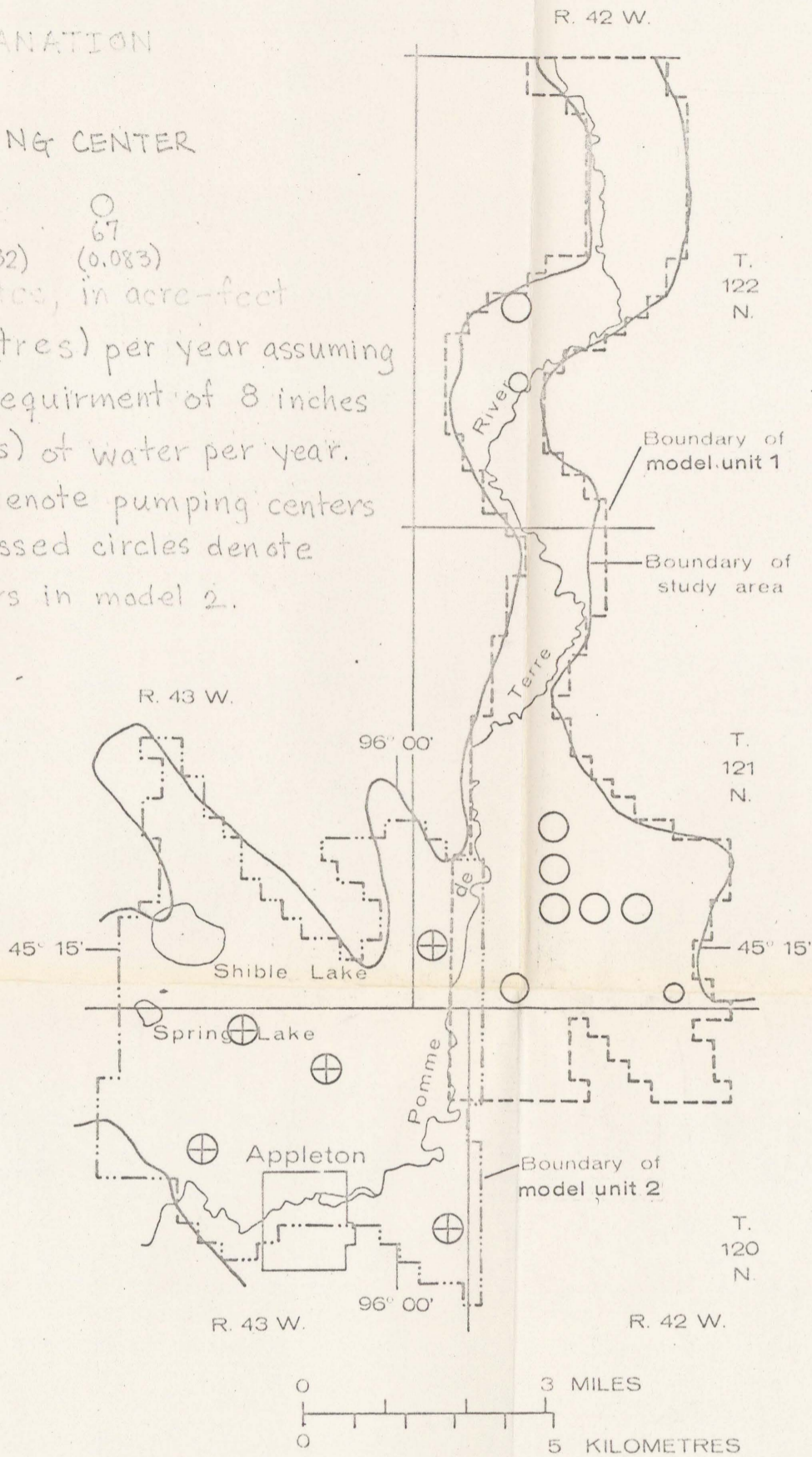
Figure 14-- Locations and withdrawal rates of present pumping centers tapping the surficial outwash aquifer.
