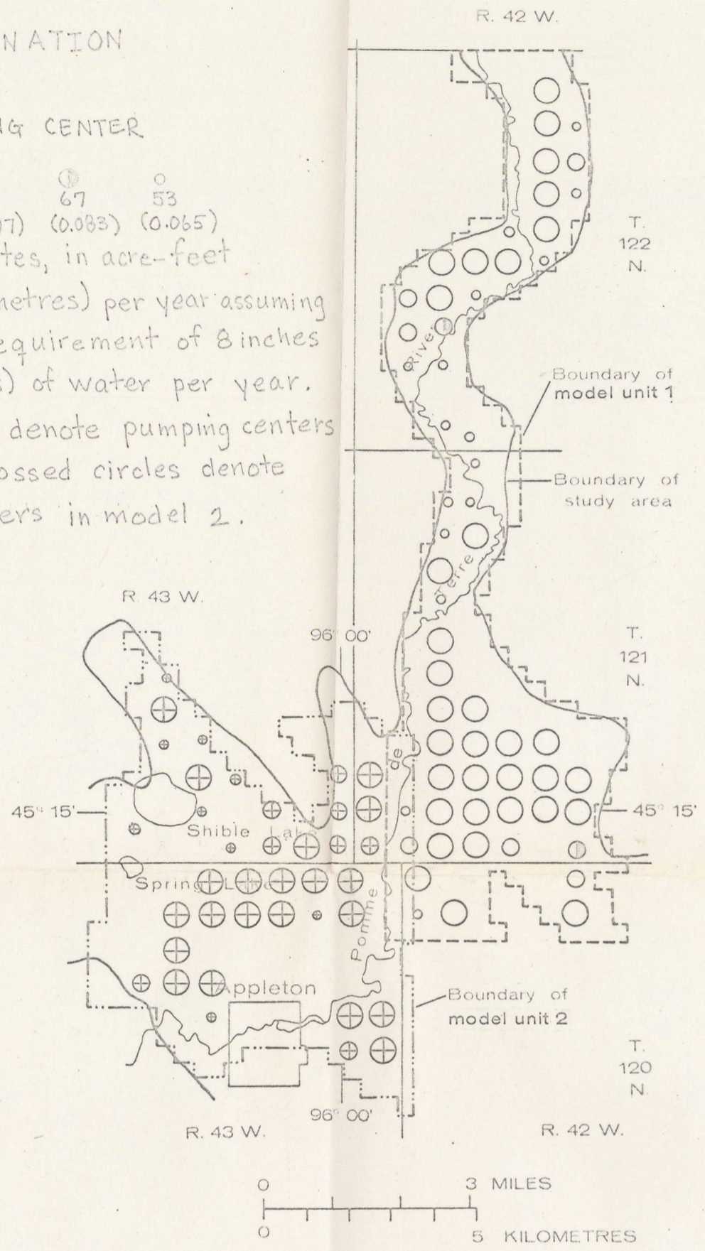
Figure 15.-- Locations and withdrawal rates of pumping centers for a maximum (hypothetical) development plan of the surficial outwash aquifer.
