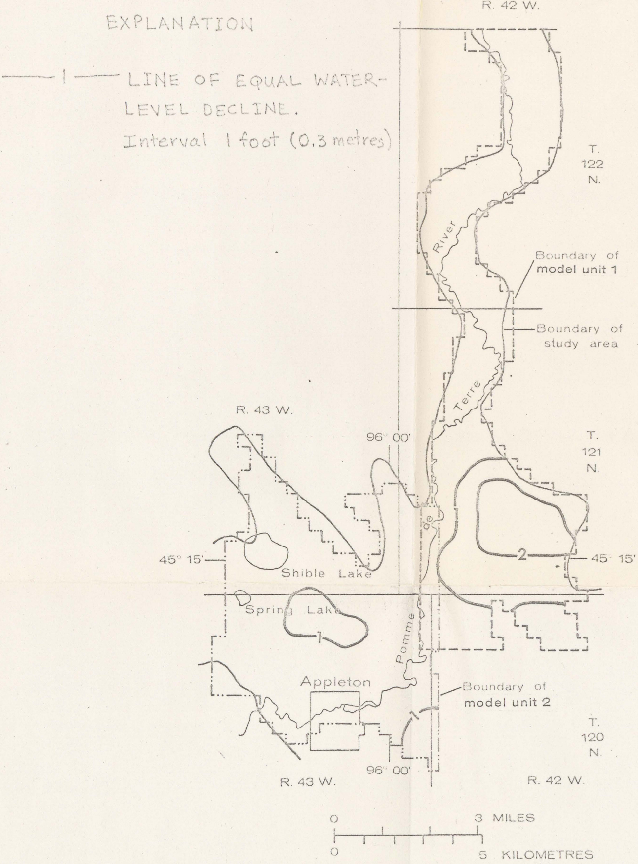
Figure 16— Predicted water-level declines after 20 years under present development [withdrawals of 1,410 acre-feet (1.74 cubic hectometres) of water per year].
